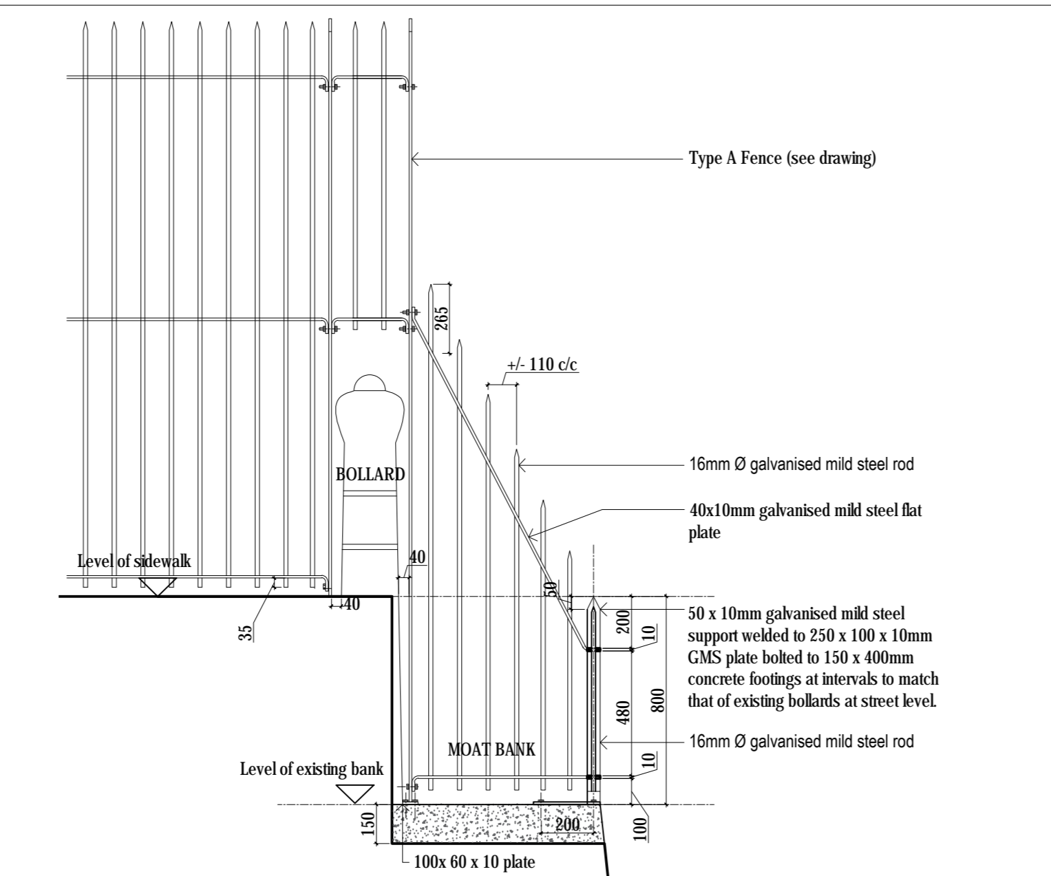
FENCE LINK FROM MOAT TO STREET Scale 1:20
