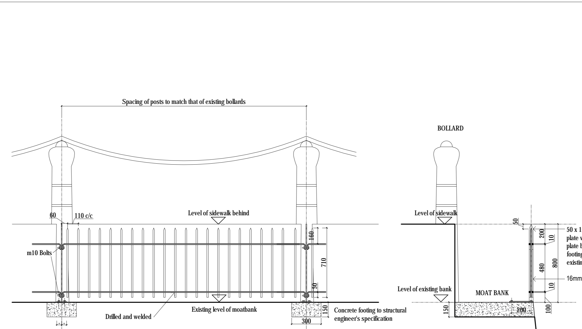
FENCE TYPE B Scale 1:20
