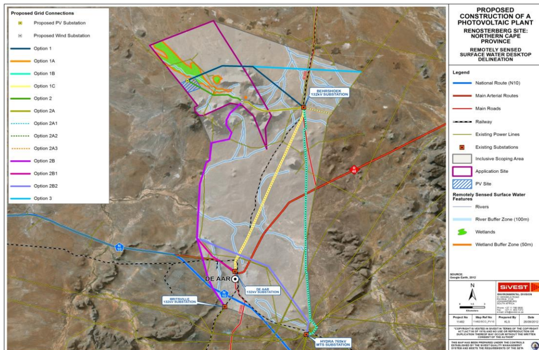
Figure 16: Google Earth Remotely Sensed Surface Water Resources for the Renosterberg all inclusive scoping area.
