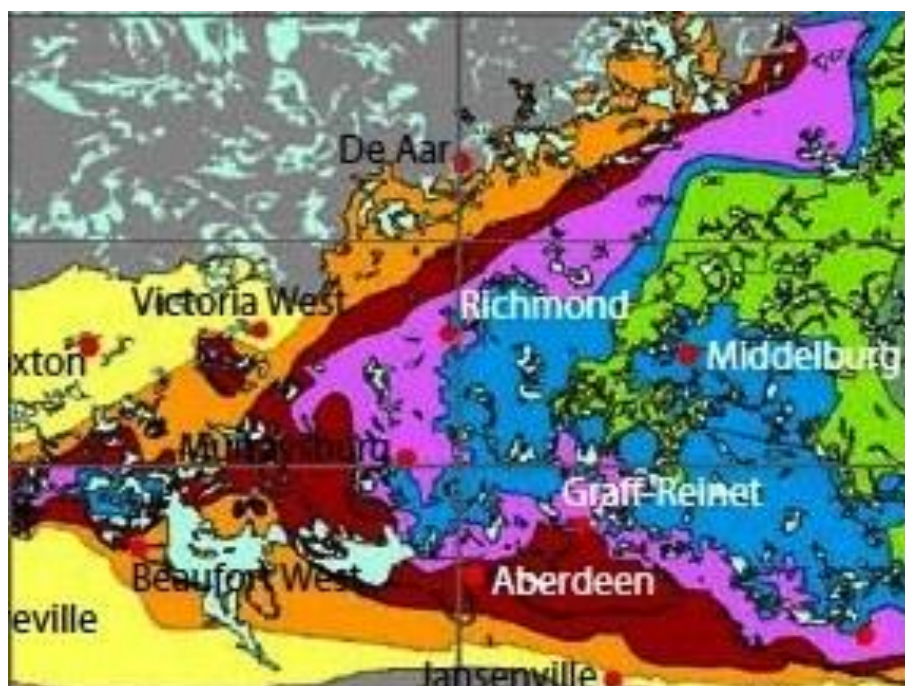
Figure 46: Abstract from recent fossil assemblage zone map for the Main Karoo Basin published by Van der Walt et al. (2010). The study region to the north and east of De Aar is assigned here to the Pristerognathus Assemblage Zone (orange), with the overlying Tropidostoma Assemblage Zone (red) only appearing well to the southeast. It is likely that the map will be refined in future in the light of new vertebrate fossil discoveries.
