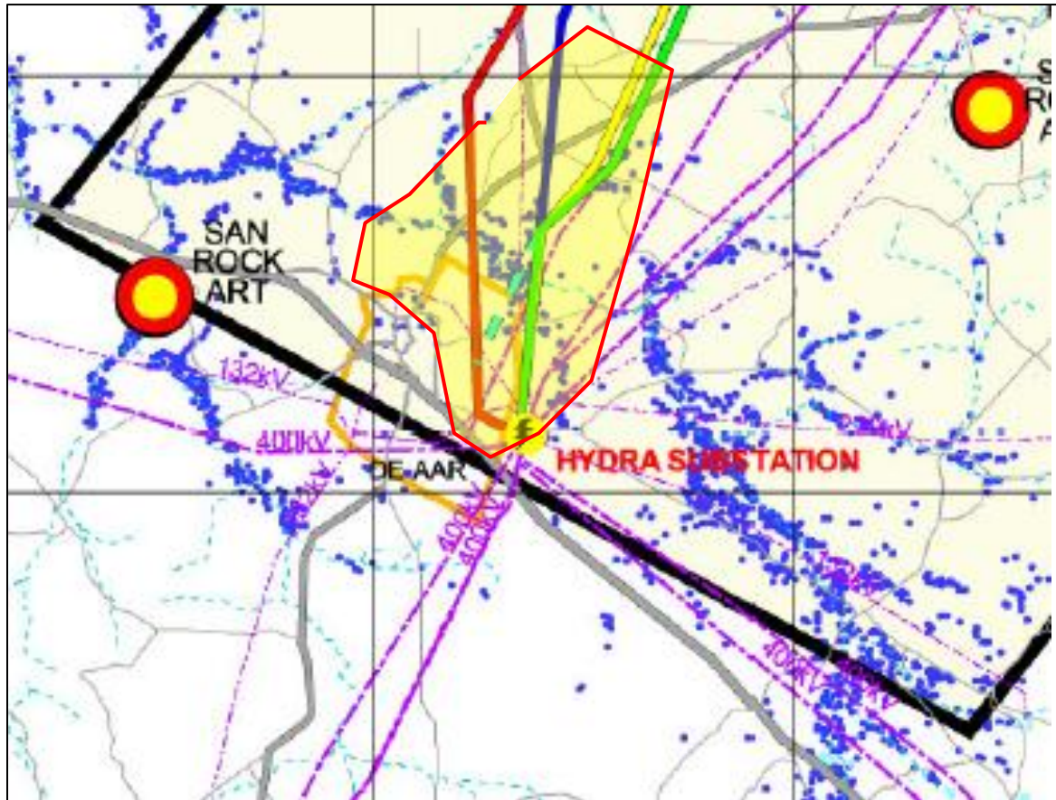
Figure 38: The greater De Aar region indicating San Rock Art finds – Blue spot indicate areas of sheet erosion (Red outline study area) (Van Jaarsveld, 2006)
