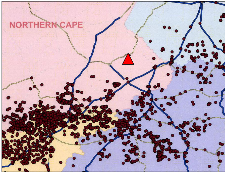
Figure 47: Distribution map of recorded vertebrate fossil sites within the Beaufort Group of the Great Karoo around the junction of the Western, Northern and Eastern Cape and the Free State (From Nicolas 2007). Note absence of documented fossil sites from the De Aar area (red triangle). This is in large part probably due to the low levels of bedrock exposure, as well as general lower abundance of fossils in the Pristerognathus Assemblage Zone. Rare vertebrate fossils have been recorded here recently during field studies by Almond (2012a).
