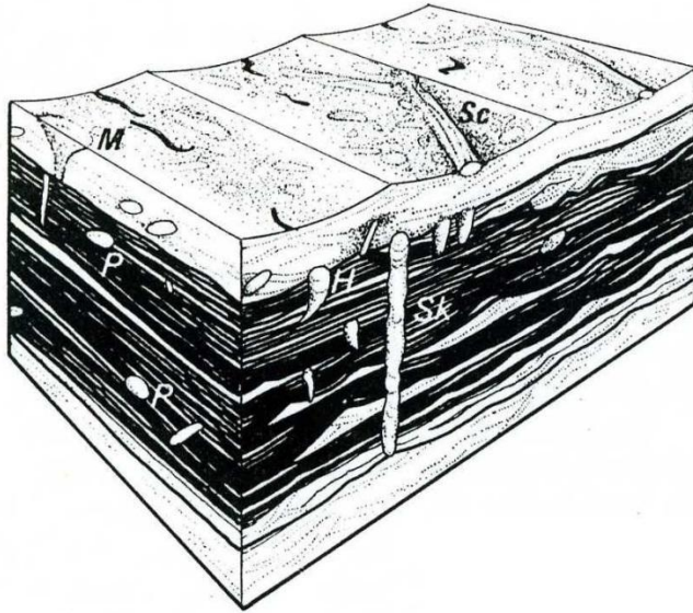
Figure 44: Schematic figure showing typical trace fossil assemblages within the storm-influenced, wave ripple laminated Carnarvon facies of the Waterford Formation (From Rust et al. 1991). Ichnogenera shown here include vertical burrows Monocraterion (M), Skolithos (Sk) and Rosselia or Histioderma (H) as well as horizontal burrows Planolites (P) and Palaeophycus (Sc).
