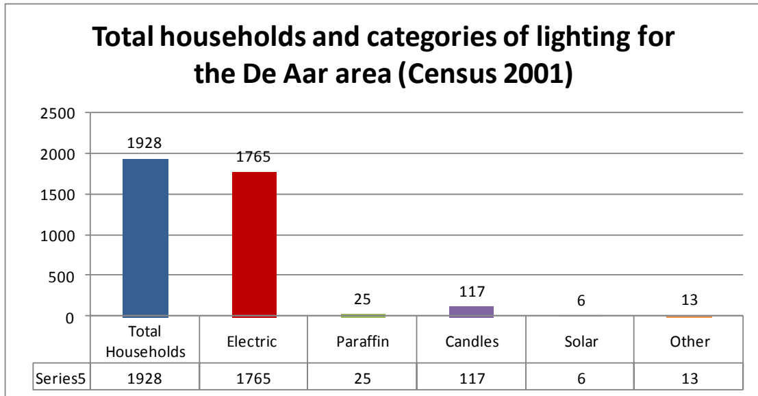
Figure 60. Energy Usage for Lighting by Category for the De Aar Area (Census 2001)
