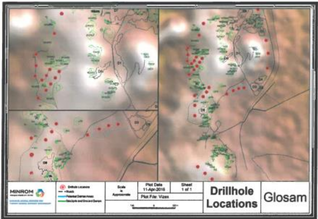
FIGURE 5: DRILLHOLE LOCATIONS.
