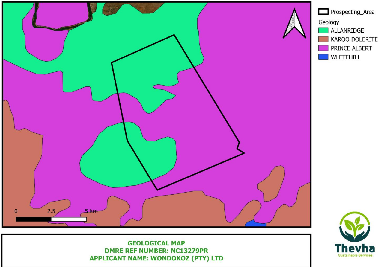
Figure 9: Geological map
