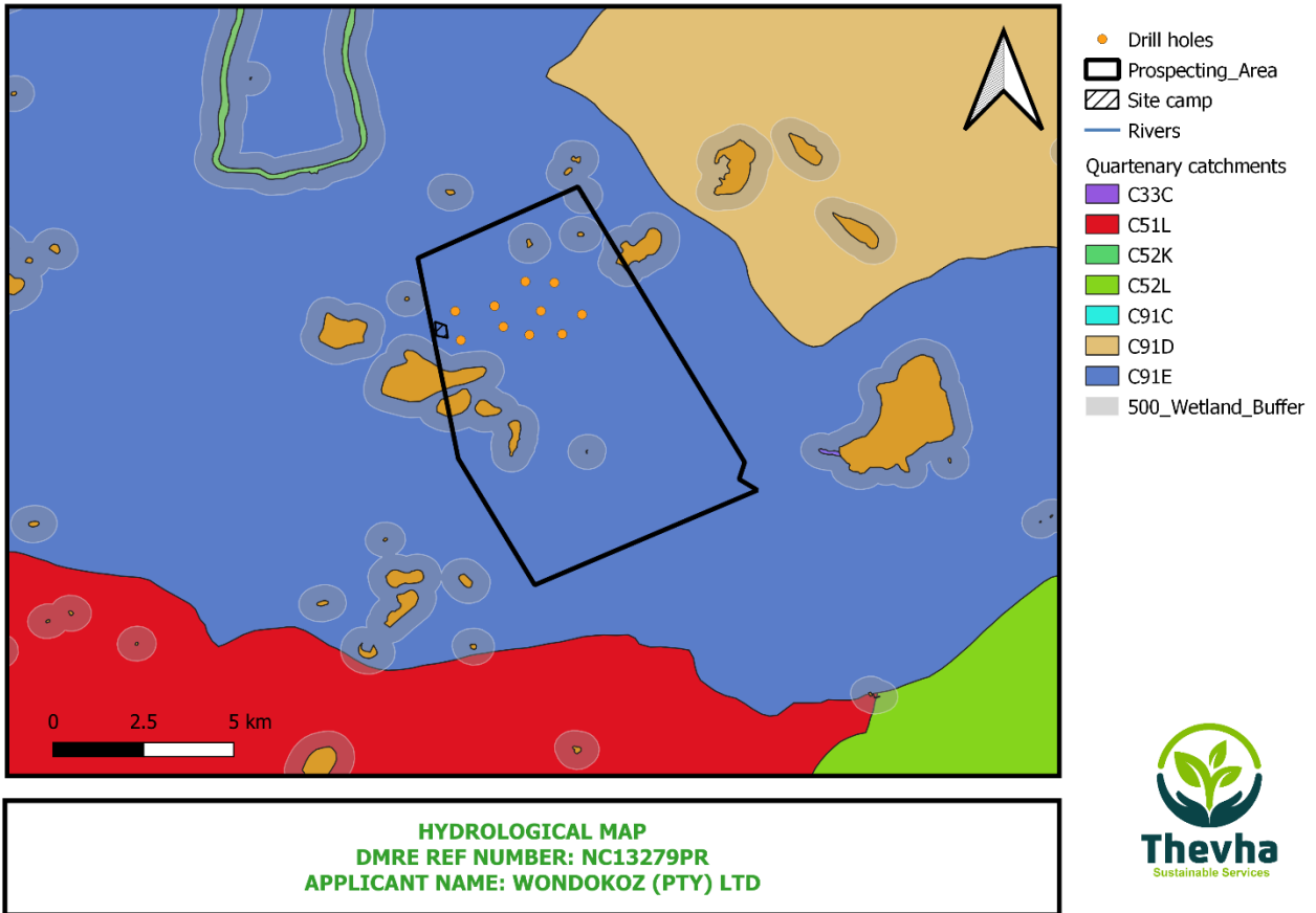
Figure 14: Hydrological map
