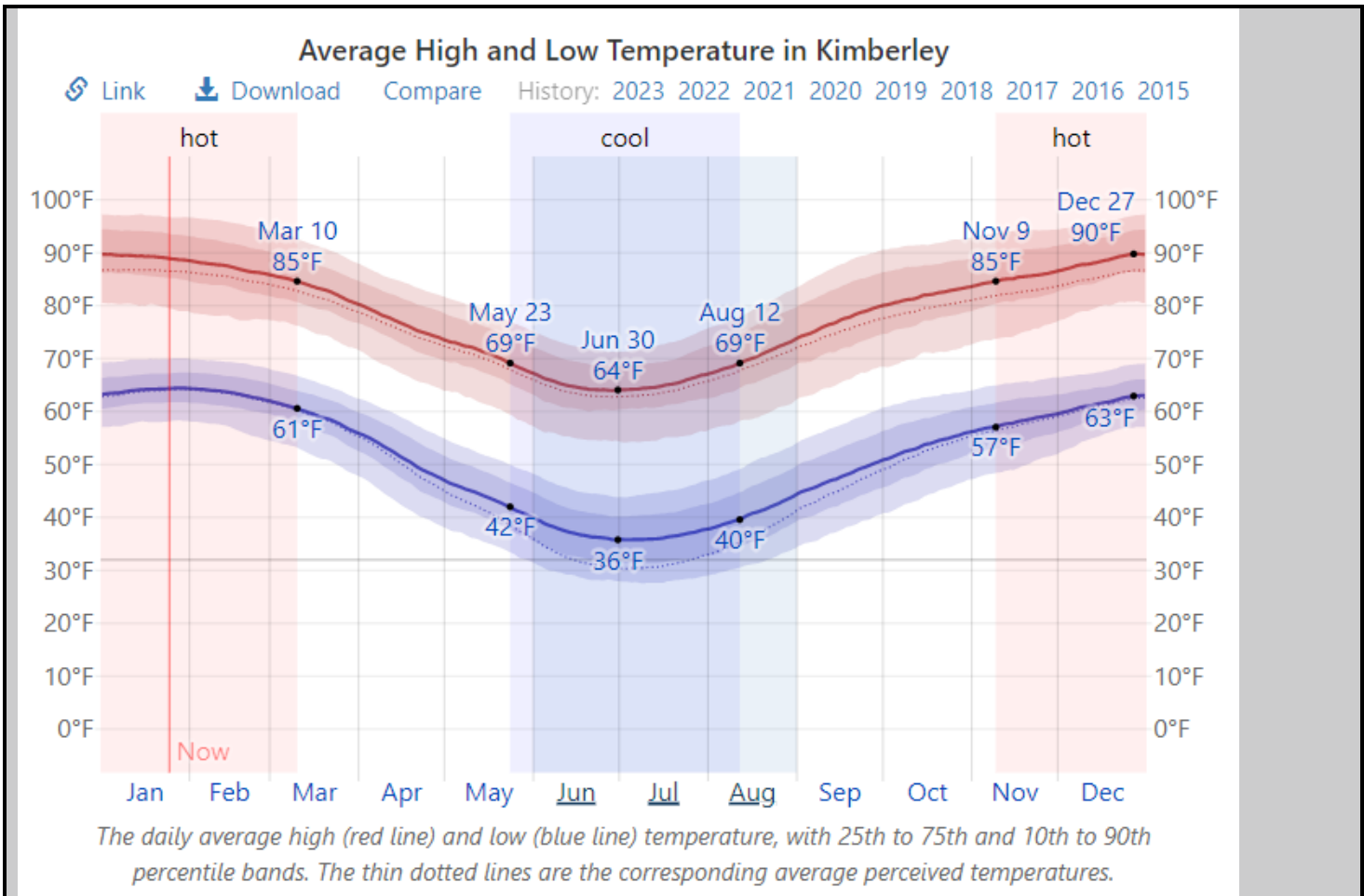
Figure 13: The daily average high (red line) and low (blue line) temperature, with 25th to 75th and 10th to 90th percentile bands. The thin dotted lines are the corresponding average perceived temperatures
