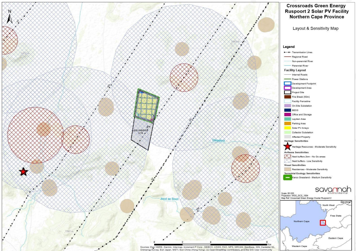
Figure 2: Ruspoort 2 Layout and Sensitivity Map
