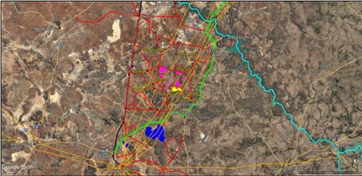
Figure 3.4: Ruspoort 1 PV Alt 1 and Alt 2 sites (yellow fill) in relation to other proposed Crossroads Phase 1 sites (pink fill), settlements, provincial boundaries (light blue), existing transmission lines (orange), the R48 (green) and study area gravel road network (red), railway line (black) and operational REFs (dark blue fill).
