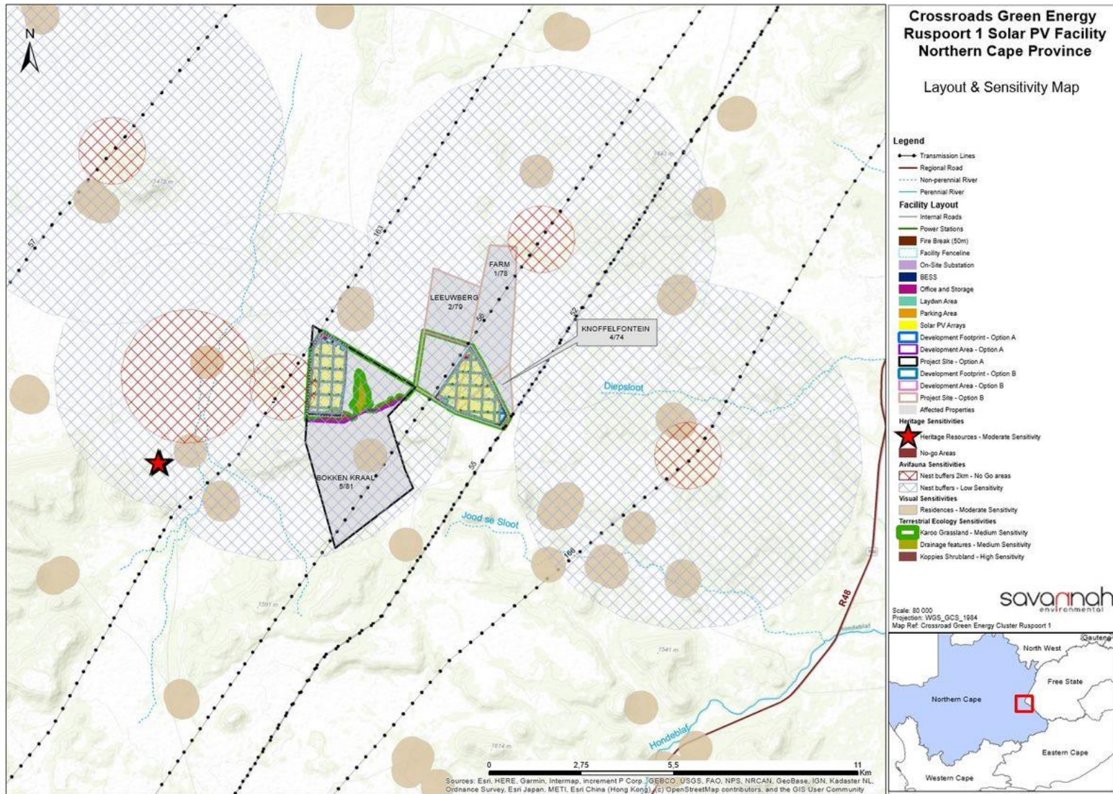
Figure 1: Environmental sensitivity and layout map of Ruspoort 1 Solar PV Facility including the onsite substation (indicated in purple)
