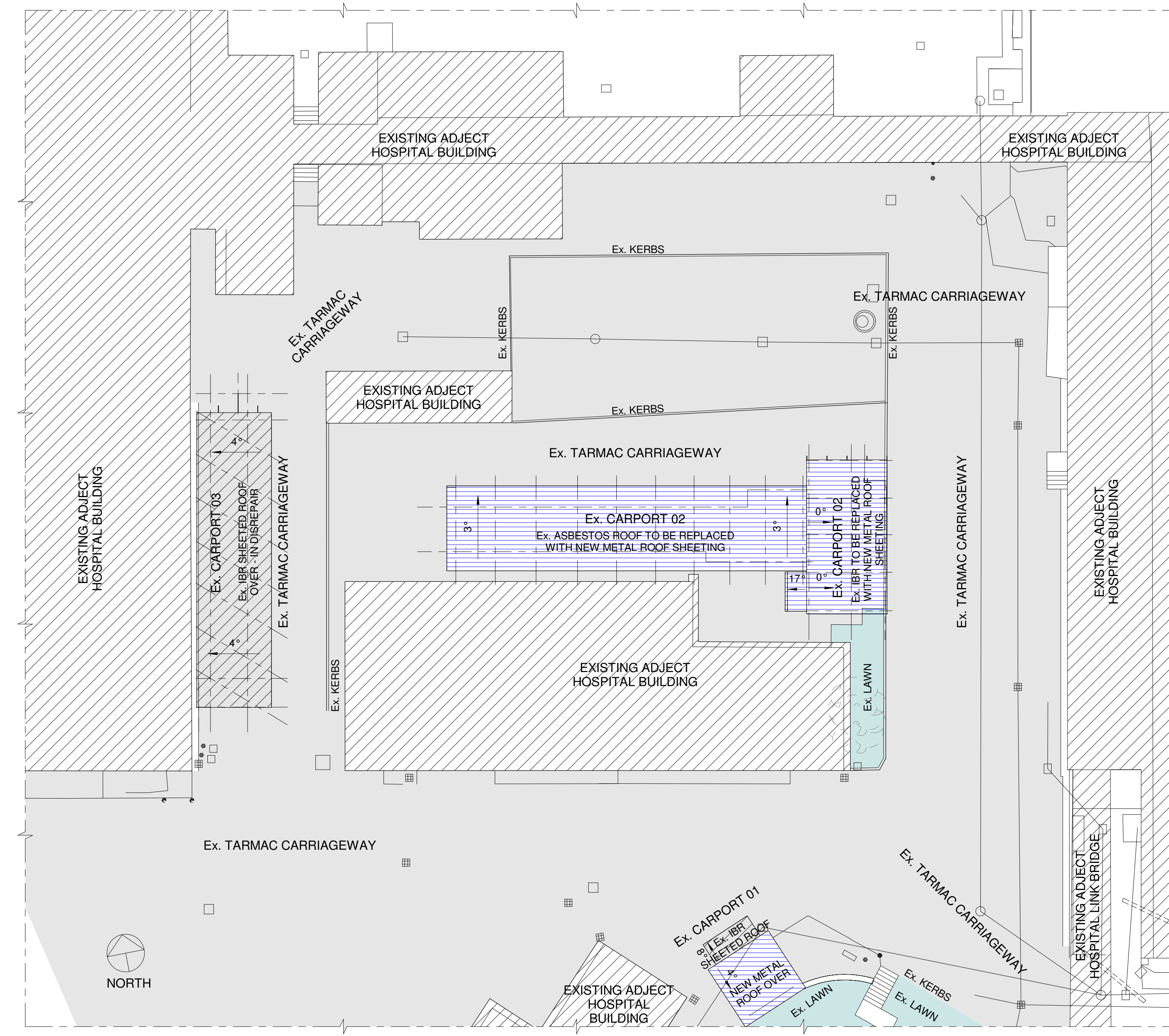
2 CAR PORTS - PORTION A - ROOF LEVEL - REFERENCE PLAN 1:200
