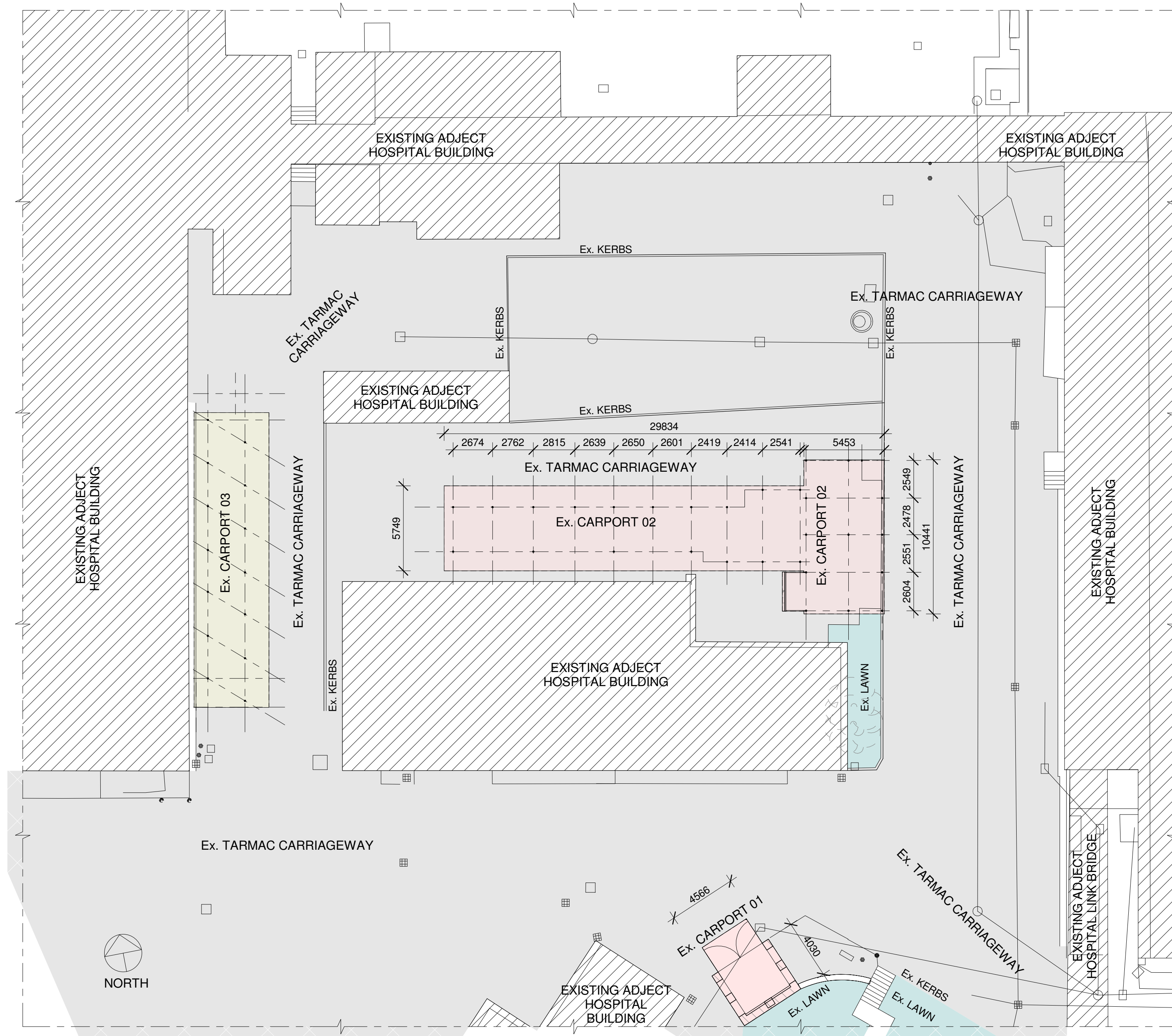
1 CAR PORTS - PORTION A - CONCEPT KEY REFERENCE PLAN 1:200
