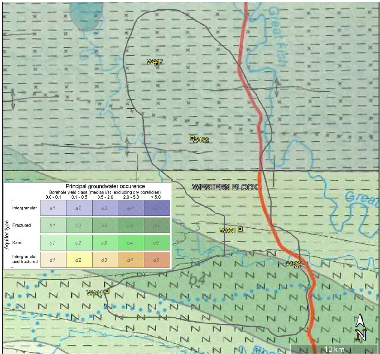
Figure 4: Regional Geohydrology - West Site
