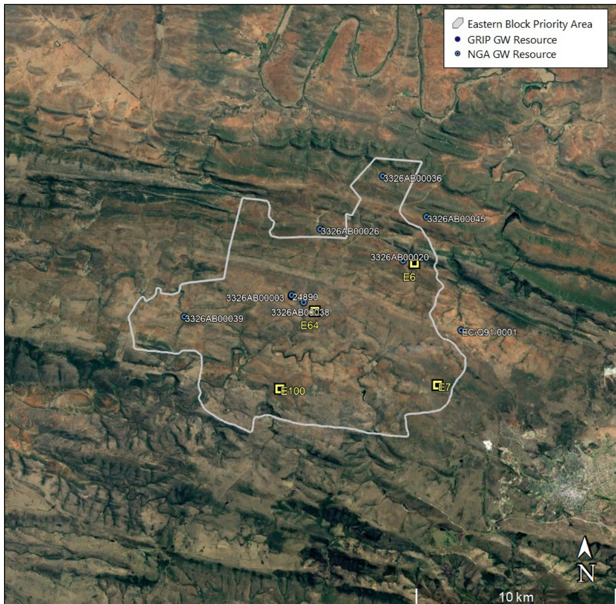
Figure 7: Existing Groundwater Resources (DWS) - East Site
