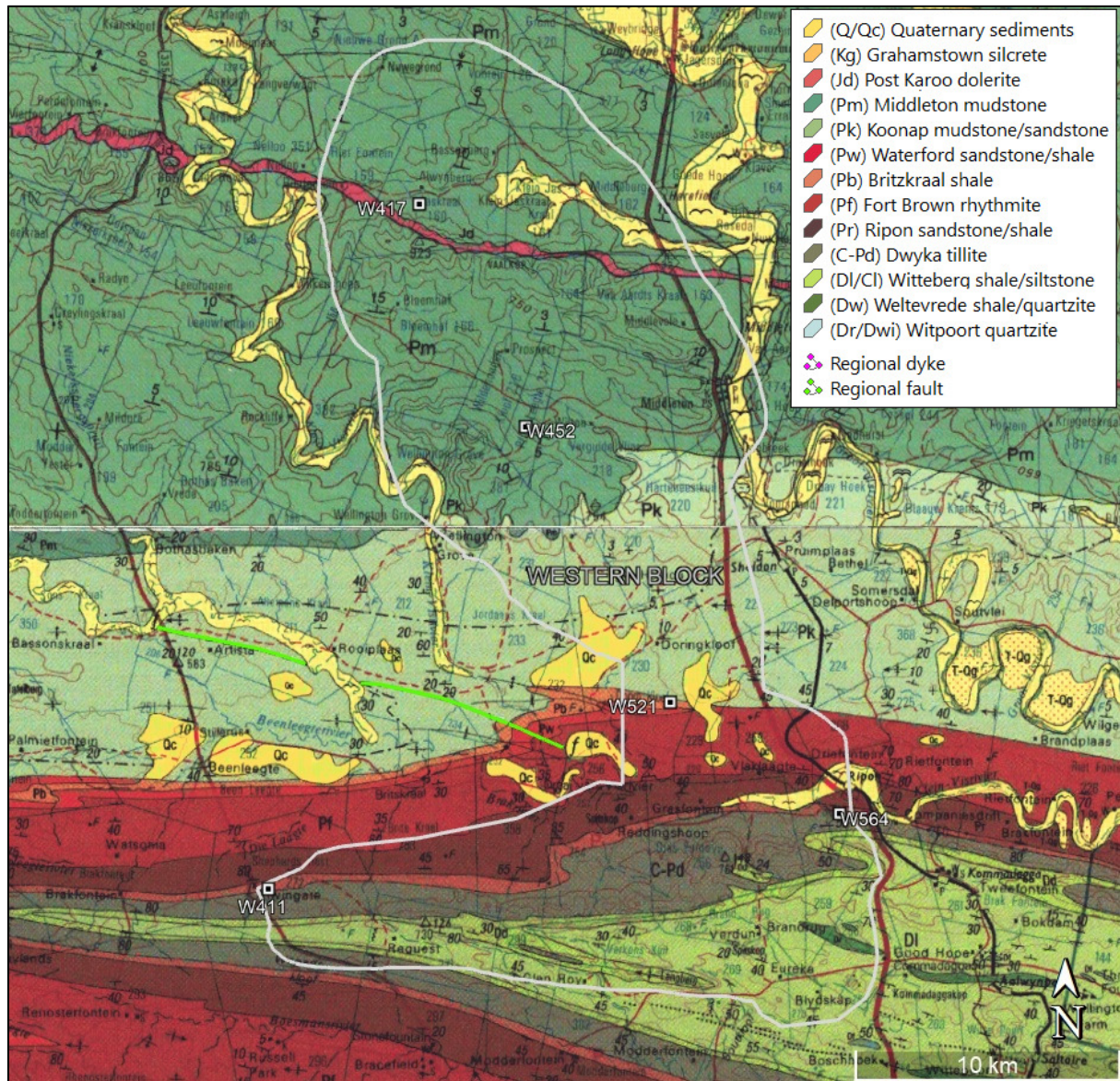
Figure 2: Regional Geology and Structures - West Site
