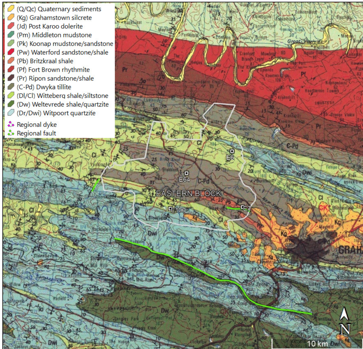
Figure 3: Regional Geology and Structures - East Site
