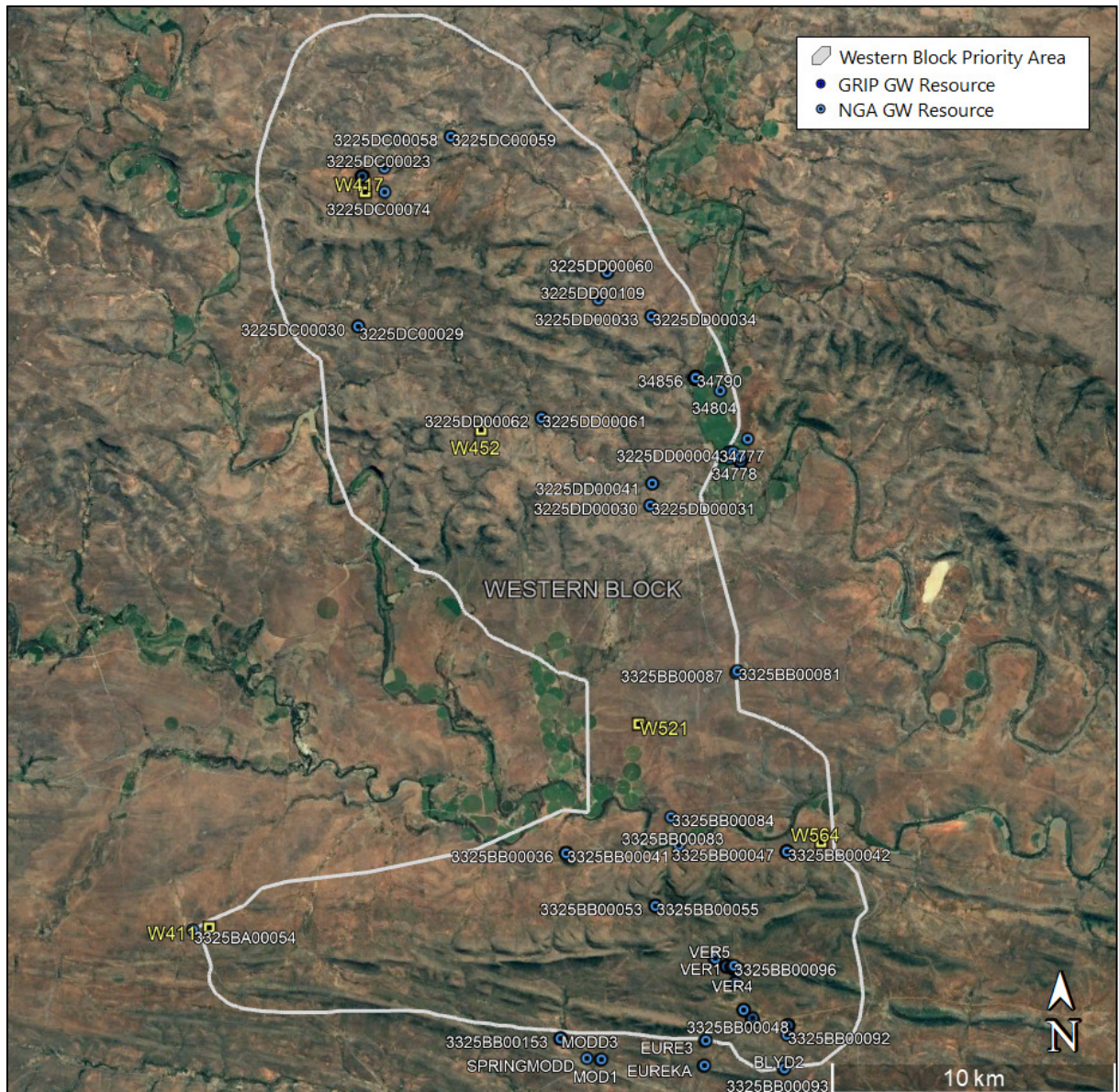
Figure 6: Existing Groundwater Resources (DWS) - West Site
