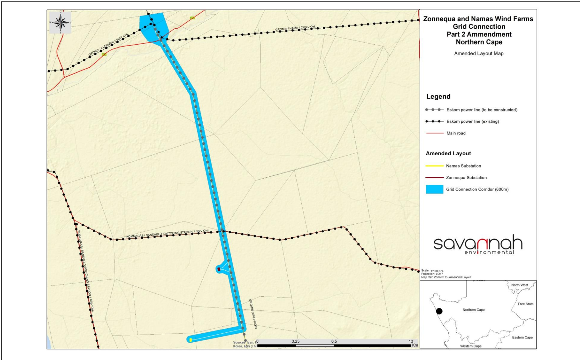
Figure 2.1: Layout map showing the grid connection corridor (600m wide) and realigned substations for the authorised Zonnequa Wind Farm
