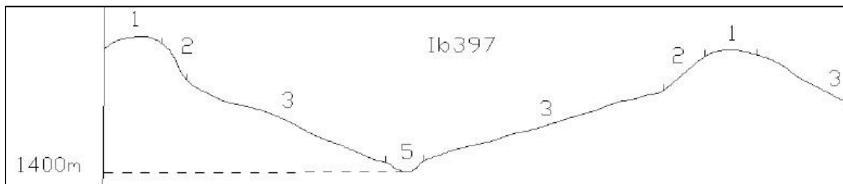
Figure 5-6 Illustration of land type Ib 397 terrain unit (Land Type Survey Staff, 1972 - 2006)
