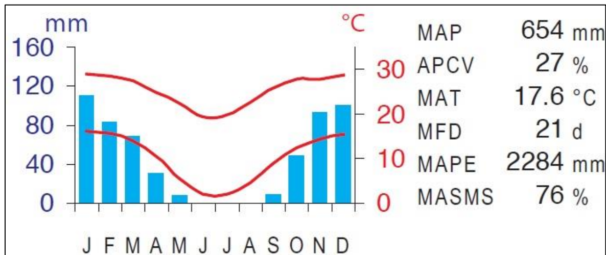
Figure 5-1 Climate for the region
