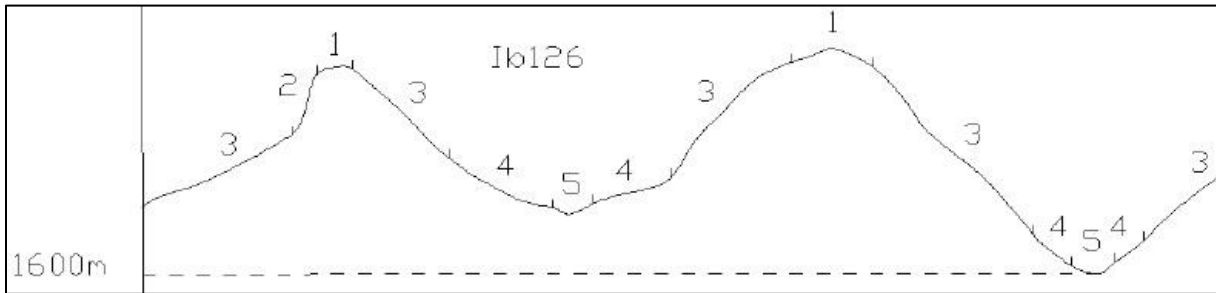
Figure 7-8 Illustration of land type Ib 126 terrain unit (Land Type Survey Staff, 1972 - 2006)
