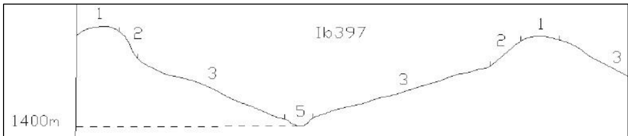
Figure 7-9 Illustration of land type Ib 397 terrain unit (Land Type Survey Staff, 1972 - 2006)
