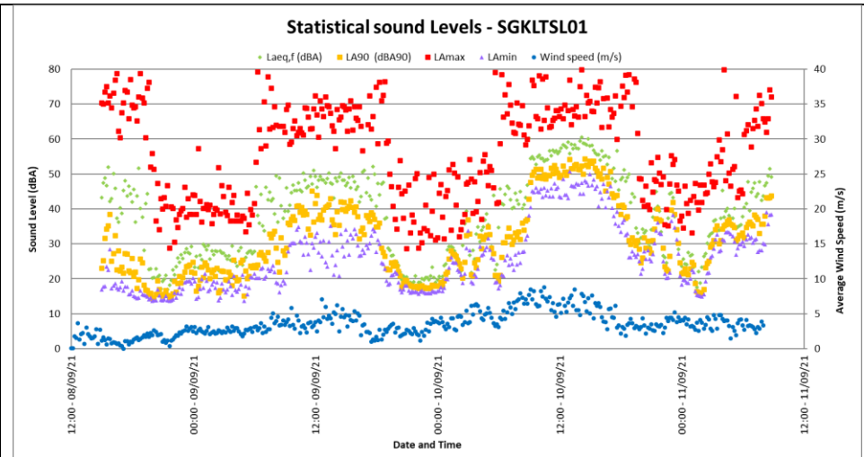
Figure 4-5: Maximum, minimum and Statistical sound levels at SGKLTSL01
