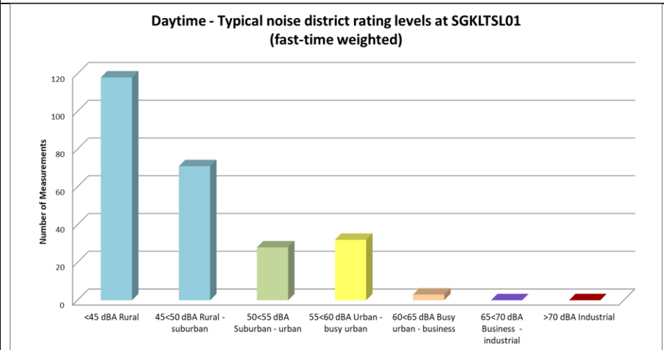
Figure 4-7: Classification of daytime measurements in typical noise districts at SGKLTSL01
