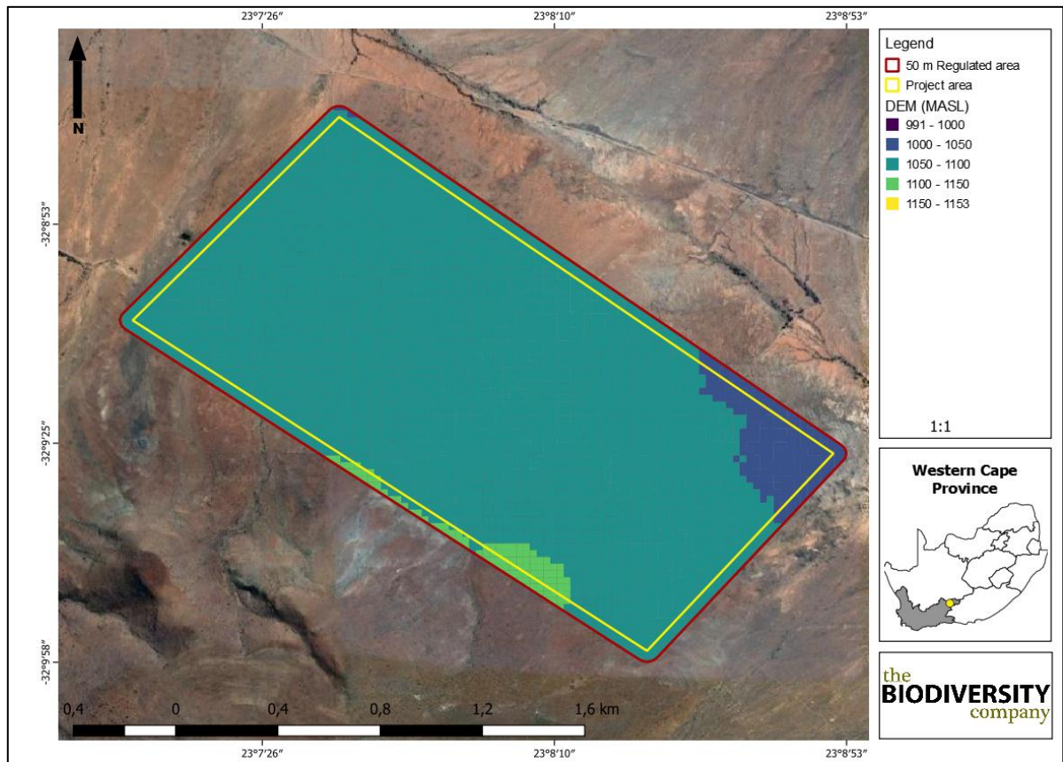
Figure 5-4 The DEM generated for the project area
