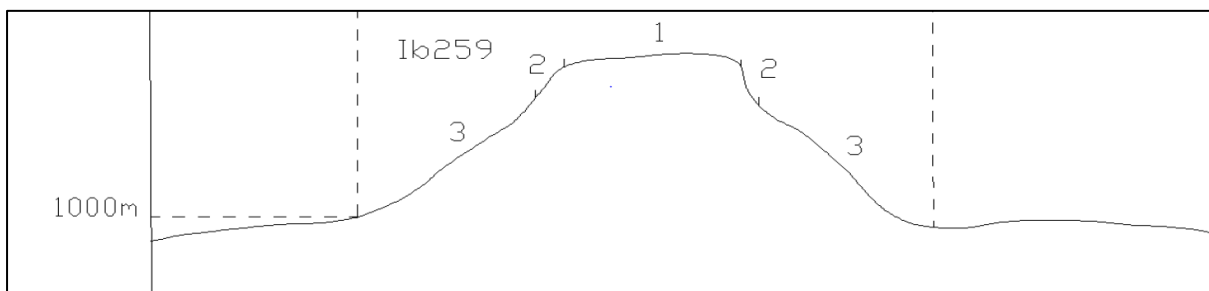
Figure 5-2 Illustration of land type Ib 259 terrain unit (Land Type Survey Staff, 1972 - 2006)
