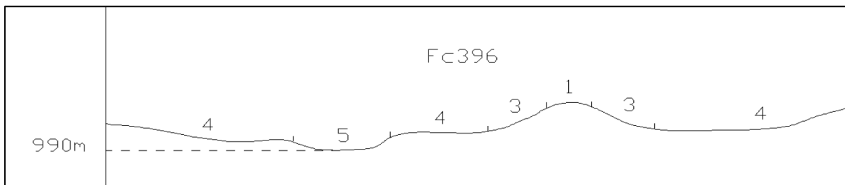
Figure 5-1 Illustration of land type Fc 396 terrain unit (Land Type Survey Staff, 1972 - 2006)
