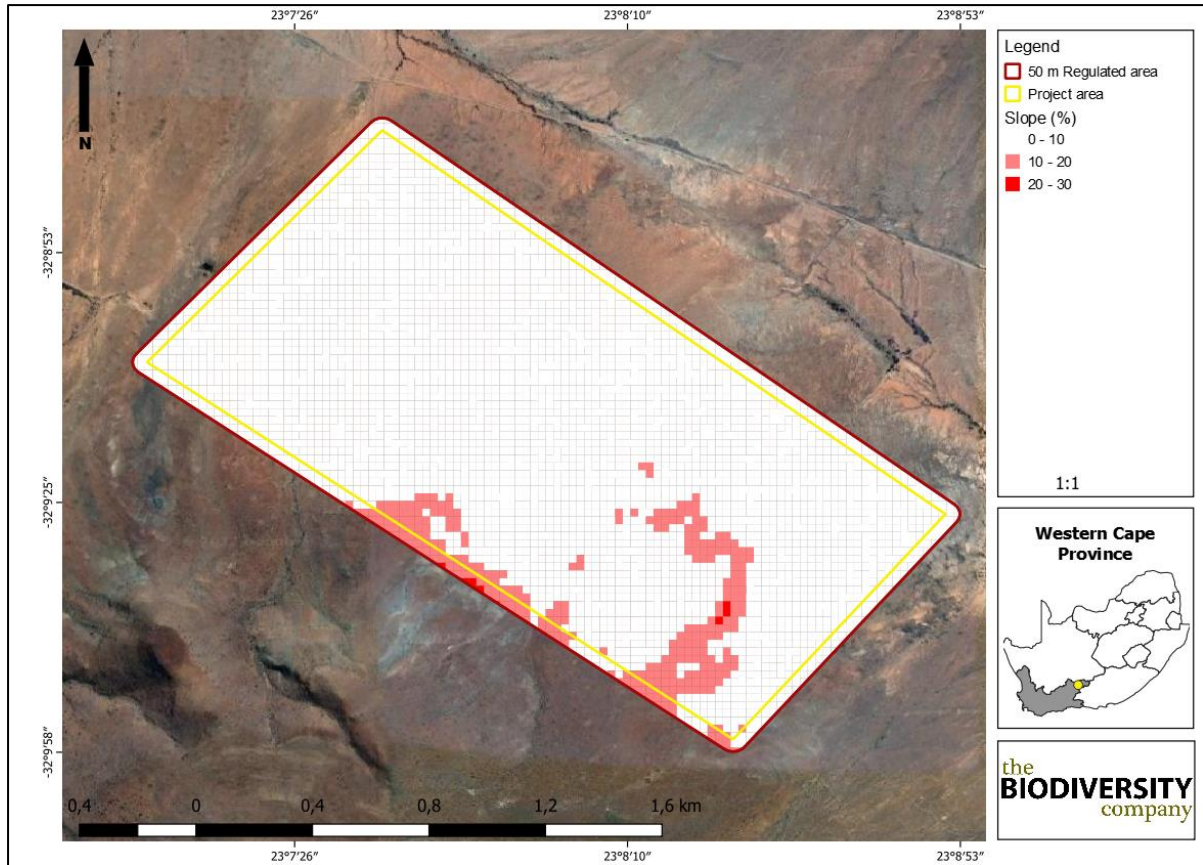
Figure 5-3 The slope percentage calculated for the project area
