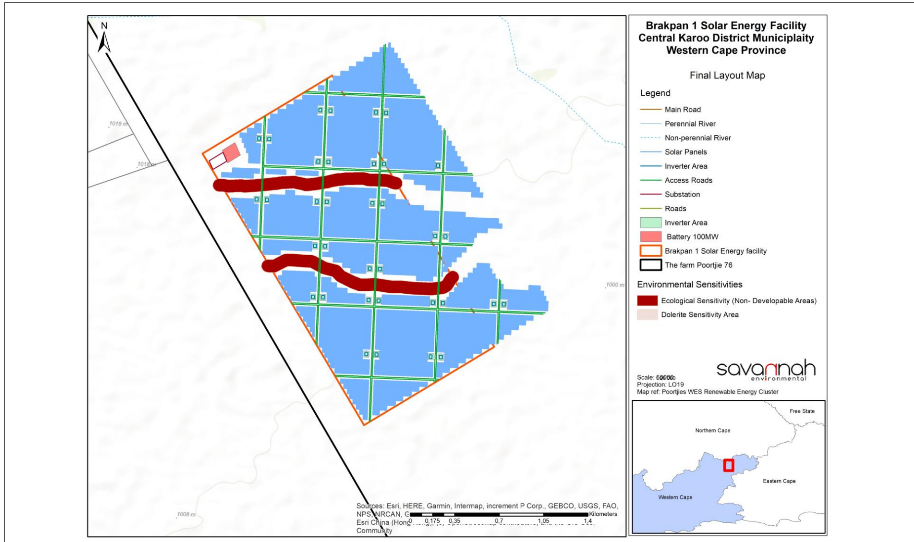
Figure 2.1: Layout of the Brakpan 1 Solar Energy facility and associated infrastructure
