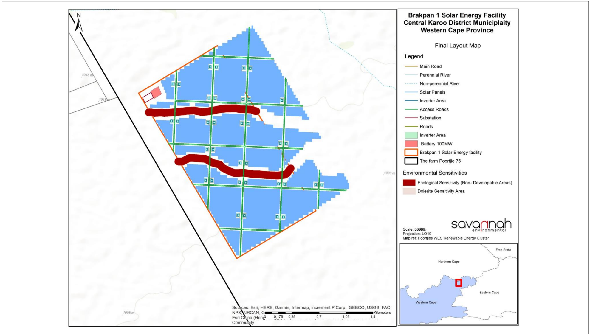
Figure 2.2: Final layout map of Brakpan 1 Solar Energy Facility development footprint (Refer also to Appendix M).
