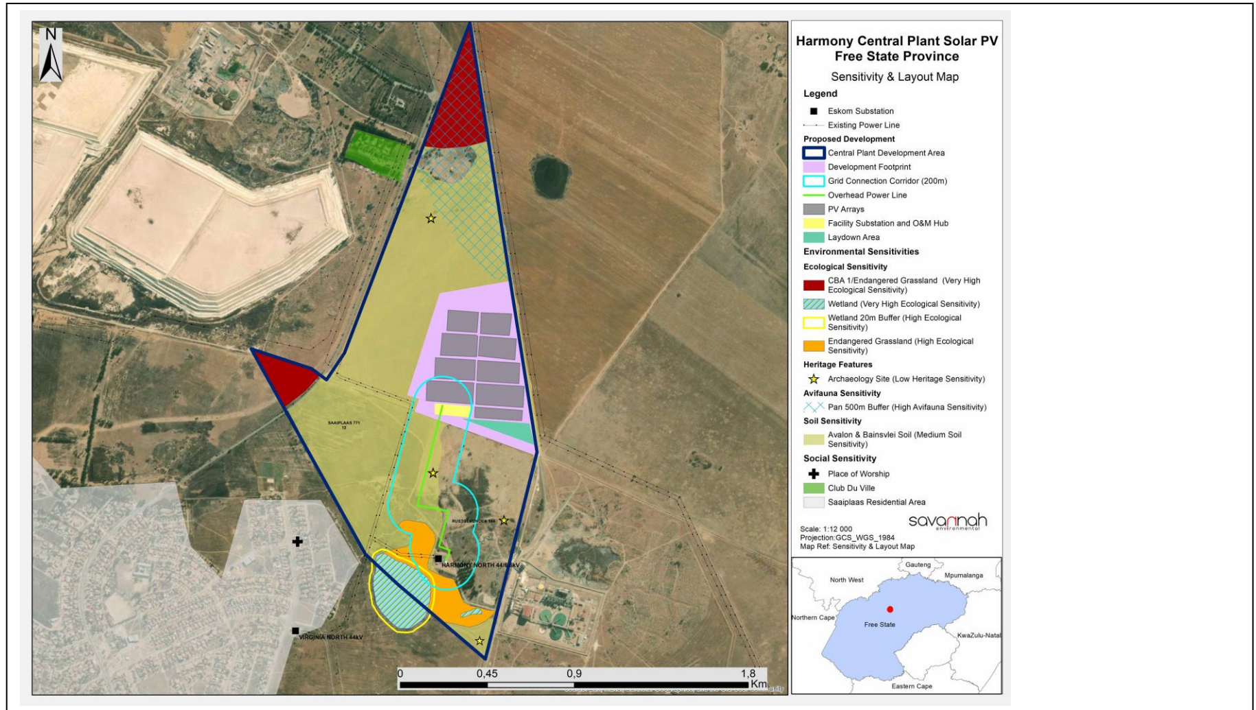
Figure 2: Layout and sensitivity map of the development footprint and grid connection corridor for the Harmony Central Plant Solar PV Facility, as was assessed as part of the EIA process (A3 map is included in Appendix O).
