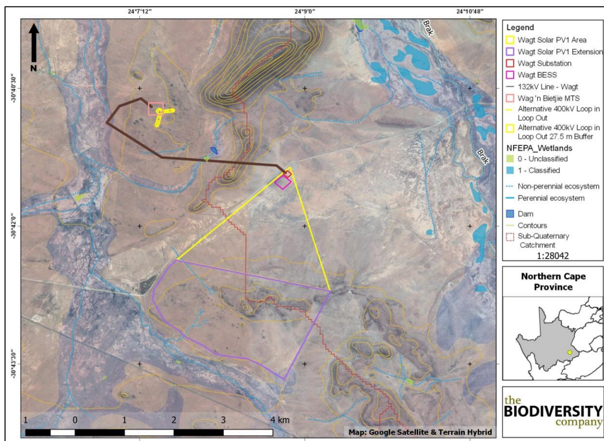
Figure 4-1 The layout for the proposed Wagt Solar PV1 facility and aquatic features
