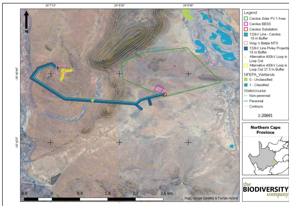
Figure 4-1 The layout for the proposed Carolus Solar PV1 facility and aquatic features
