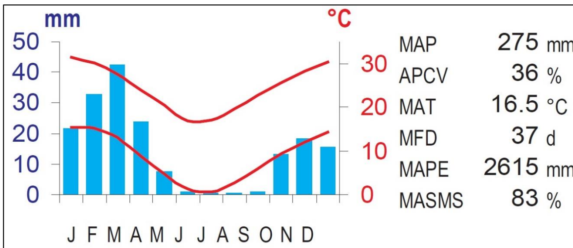
Figure 3-5 Climate for the region (Mucina & Rutherford, 2006)
