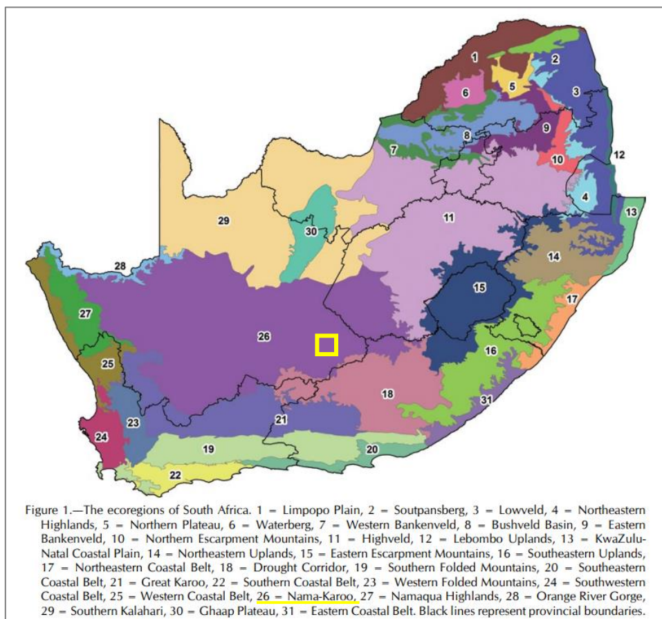
Figure 3-3 Ecoregions for the project area (yellow square) according to Kleynhans et al. (2005)
