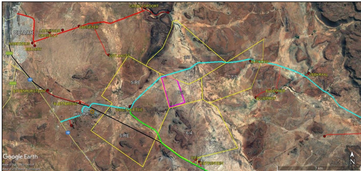
Figure 3.6: Fountain PV 1 site (pink outline) in relation to site- and adjacent properties (yellow), local settlement pattern, railway line (black), the Hydra road (blue), the Hanover Road railway road and other local roads.
