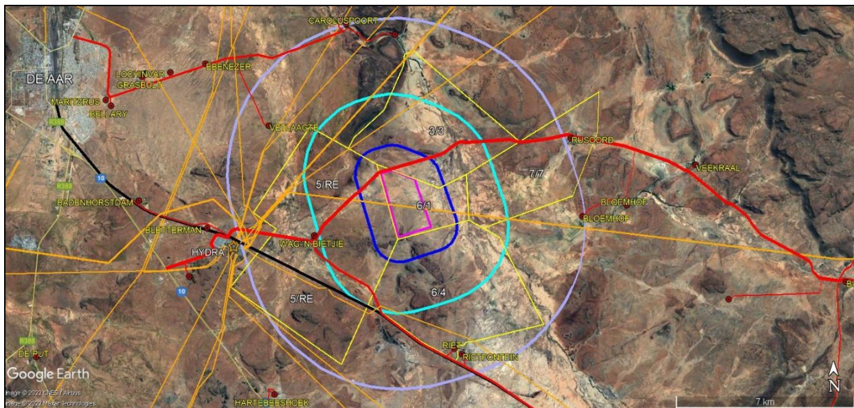
Figure 3.7: Fountain PV 1 site (pink outline) in relation to local receptors; dark blue circle indicates 1 km from site, light blue 3 km, and light purple 6 km. Also indicated are the railway line (black), local roads (red; Hydra Rd in bold), and existing Eskom lines (orange) (distances mapped from Scoping VIA 12 ).
