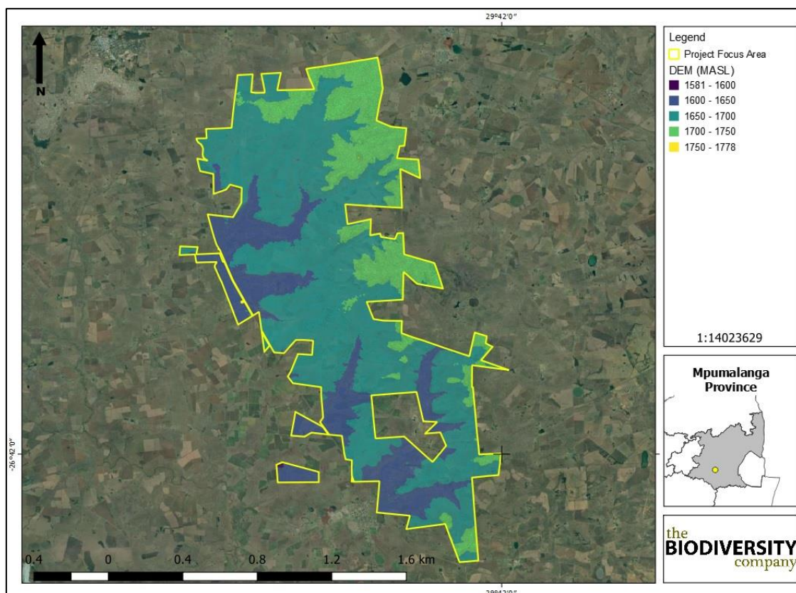
Figure 5-6 The DEM generated for the project area
