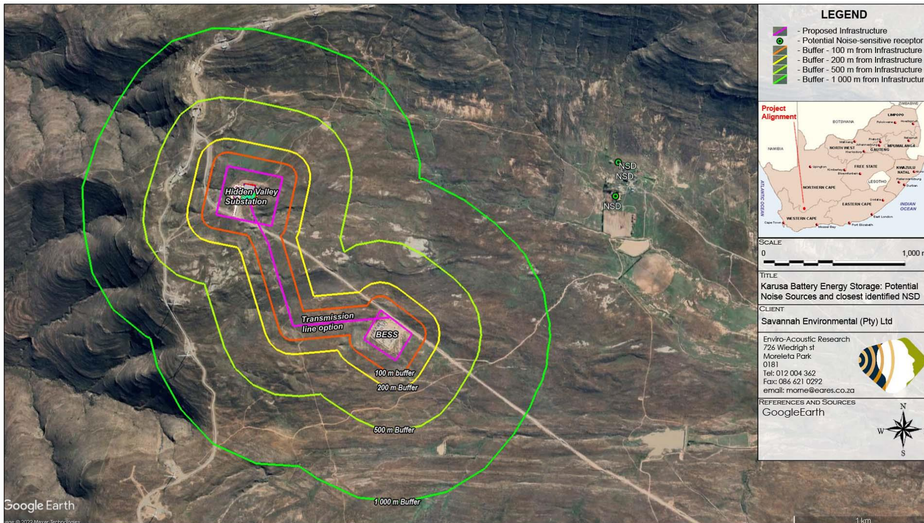
Figure 4-2: Locations of proposed BESS in relation to the identified noise-sensitive developments (receptors)
