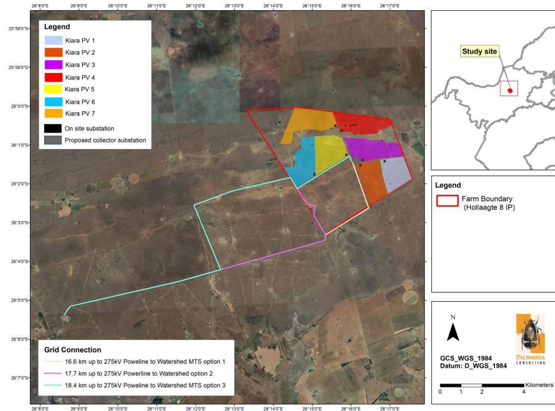
Figure 2: A satellite image illustrating the geographic position of the proposed Kiara PV 2 facility in relation to six other planned PV facilities corresponding and the proposed grid connection options.
