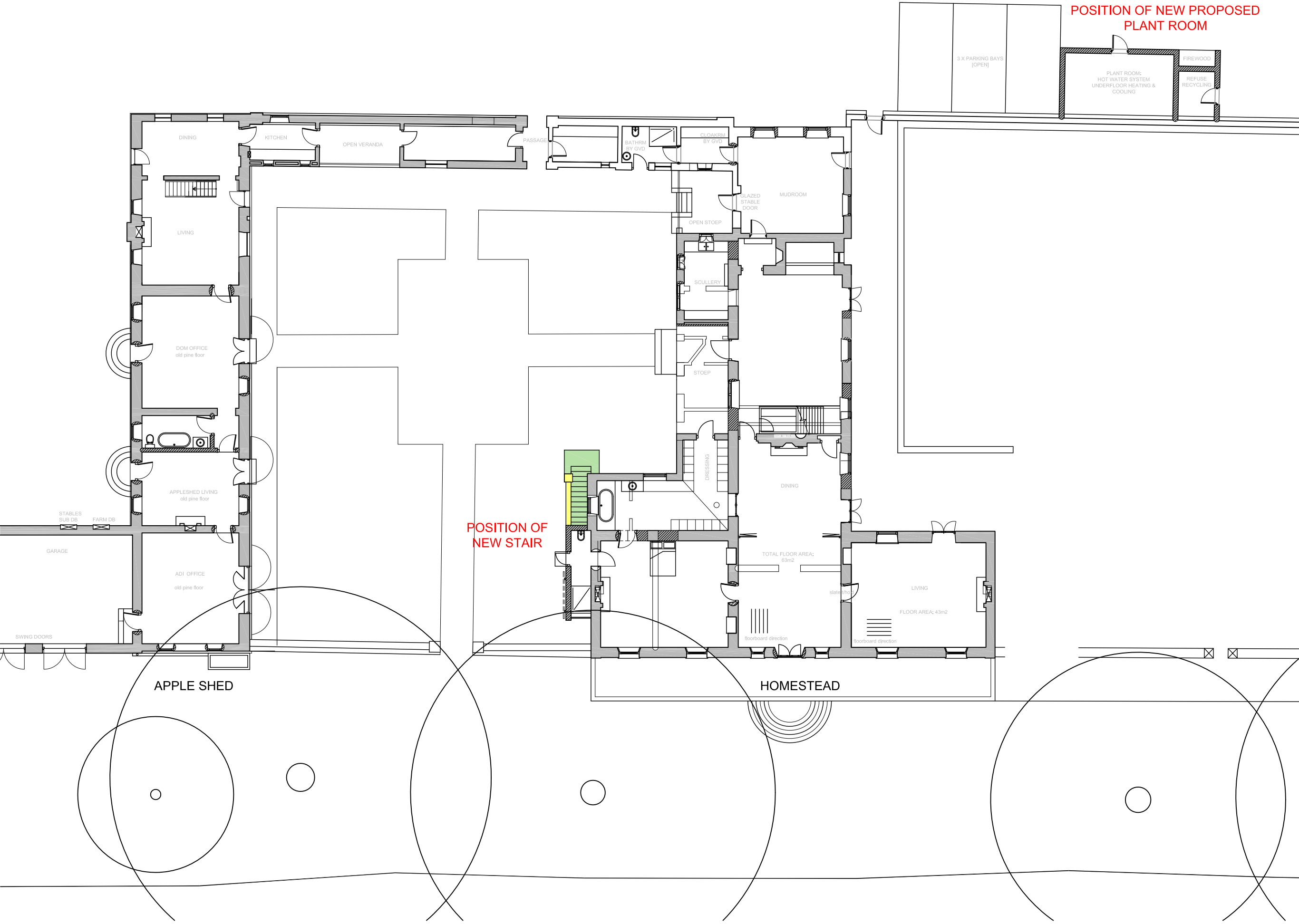
HOMESTEAD, APPLE SHED AND PLANTROOM PLAN SCALE 1:200
