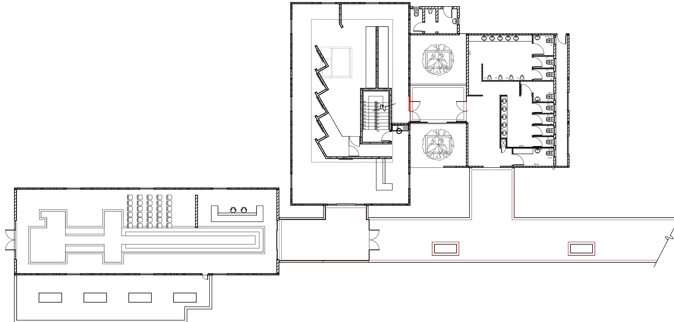
Scale 1:100 Taung Skull & Mine Museum - groundfloor sanitary fitting layout
