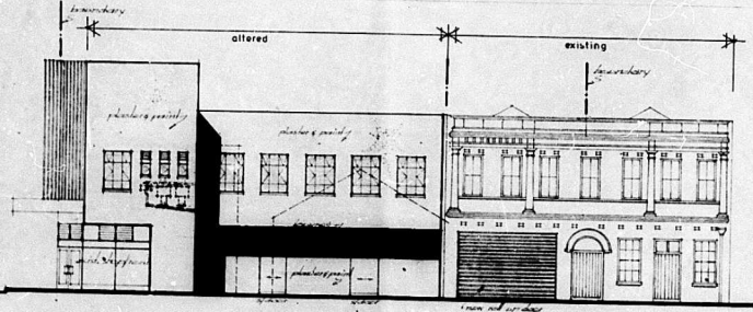
elevation from saville street
