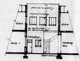
section C-C 1:100
