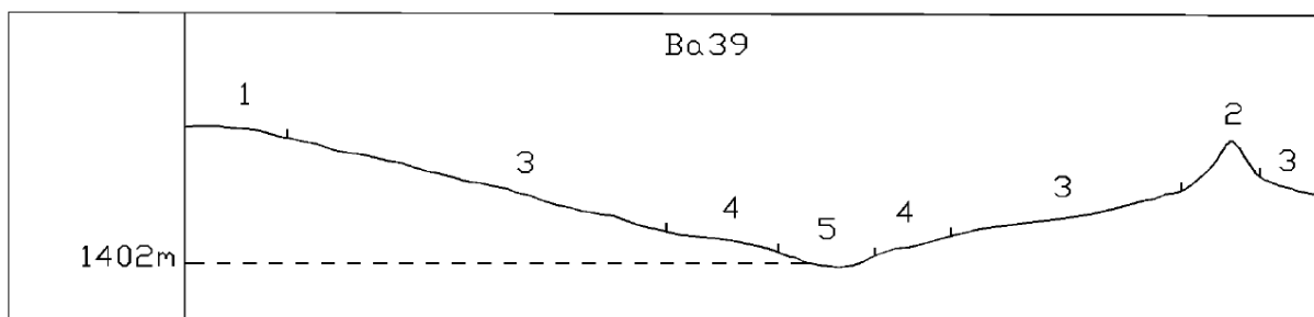
Figure 6 Terrain form sketch of Land Type Ba39
