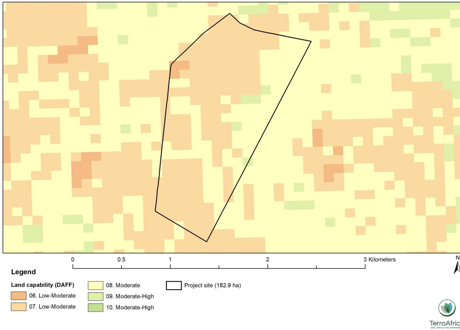
Figure 13 Land capability map of the Damlaagte project site (DALRRD, 2016)
