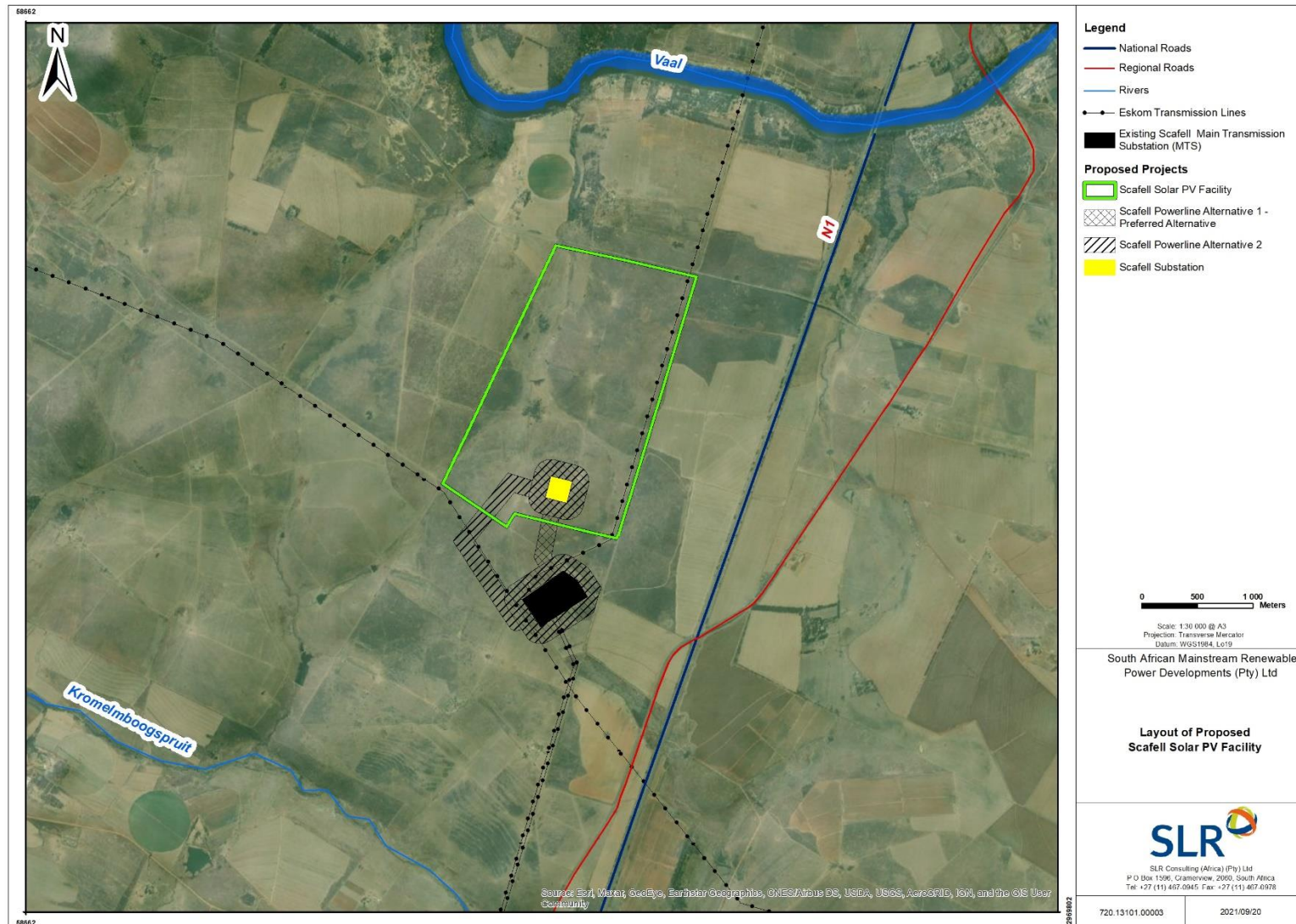
Figure 2: Location of the proposed grid connection infrastructure for the proposed grid connection infrastructure for the Scafell Solar PV Facility in relation to the surrounding area.
