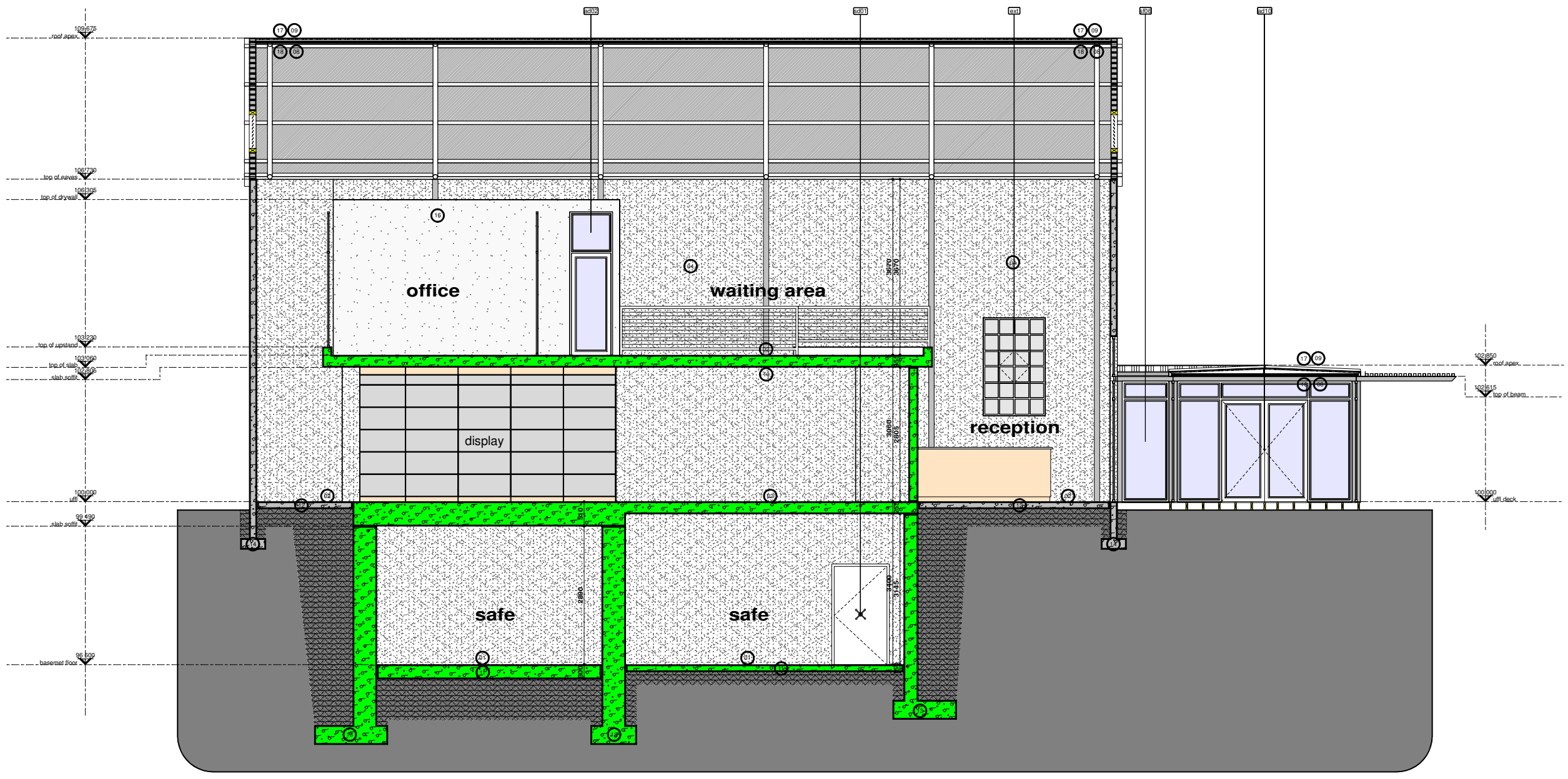
Scale 1:50 Taung Skull & Mine Museum - section a-a
