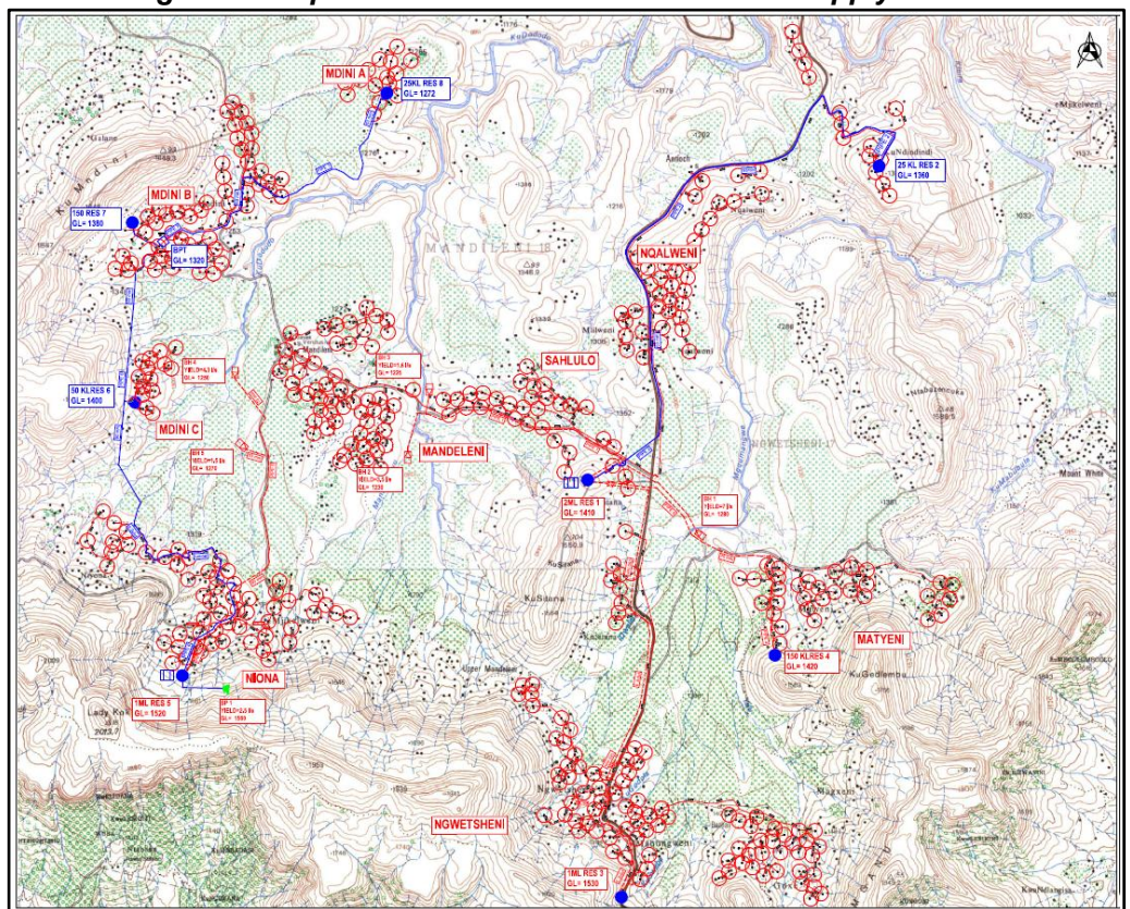
Figure 1: Proposed Umzimvubu Water 14 Water Supply Scheme
