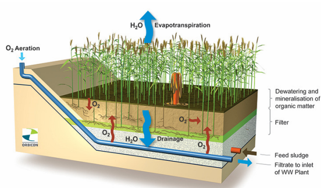
Figure 5 – Typical Reed Bed
