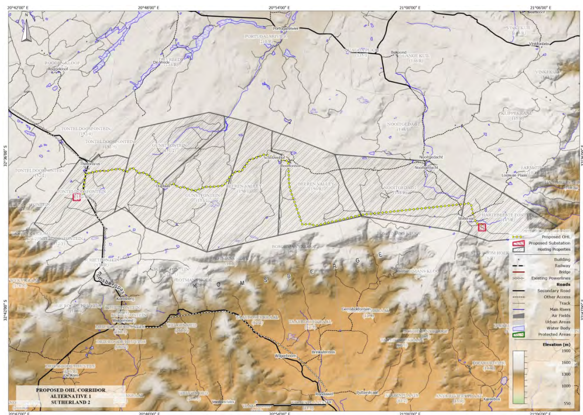
Figure 1-1 Proposed Alternative 1 132 kV overhead line and substations associated with the Sutherland 2 WEF.
