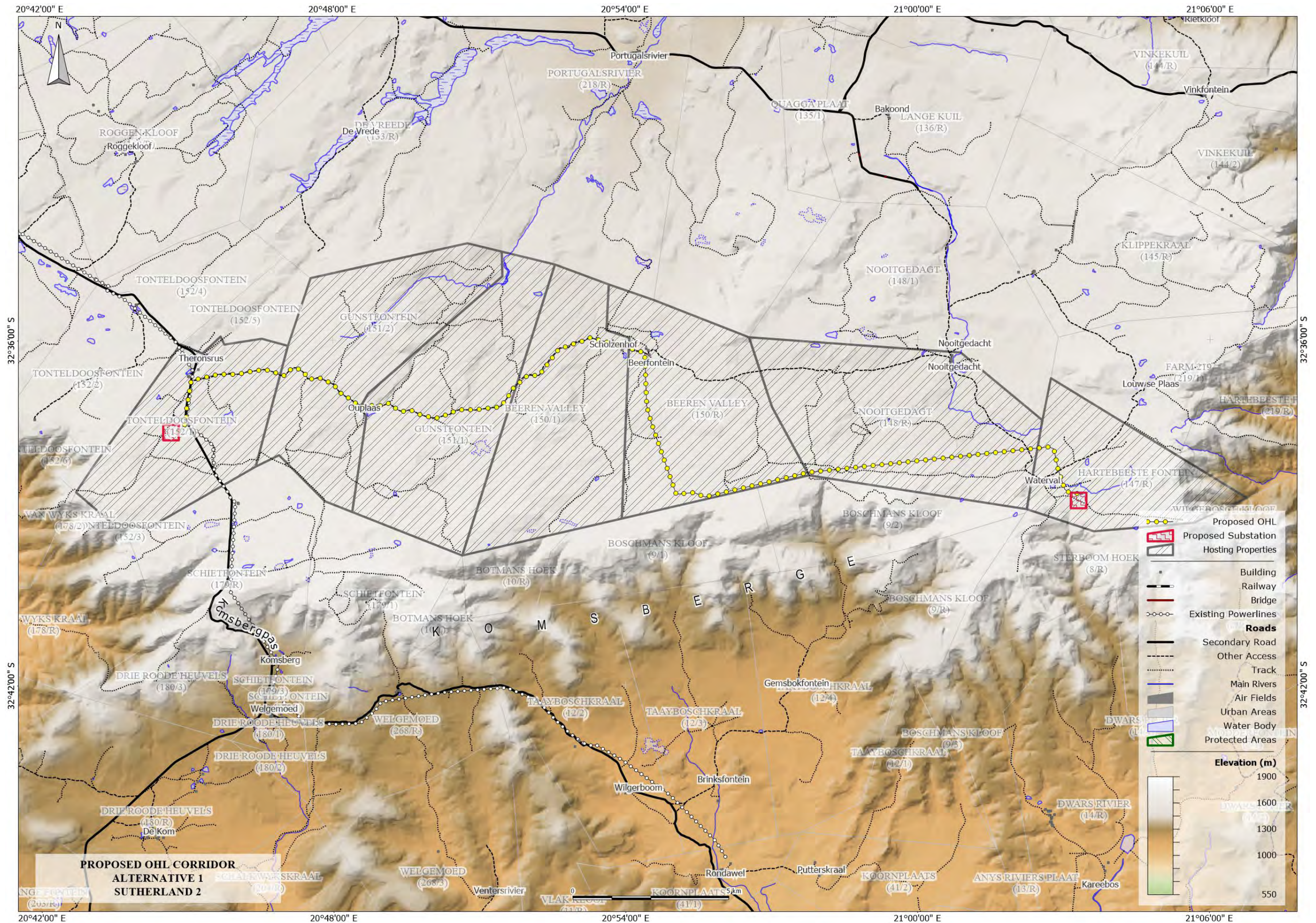
Map 1 Proposed Alternative 1 of the 132 kV overhead line and substations associated with the Sutherland 2 WEF.
