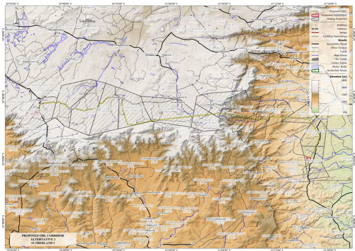
Figure 1-2 Proposed Alternative 2 132 kV overhead line and substations associated with the Sutherland 2 WEF.
