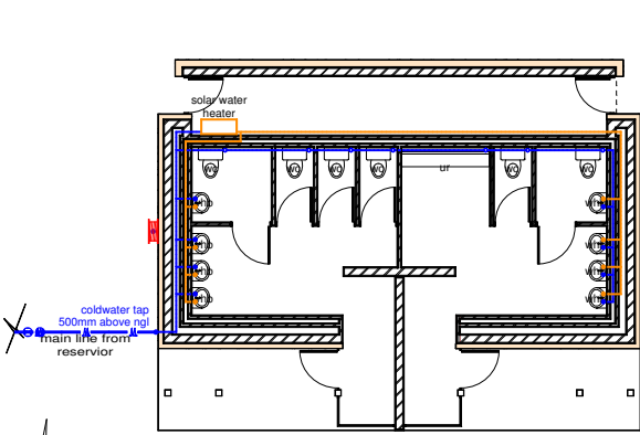
Picnic Site Ablutions - water reticulation plan
