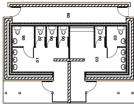
Scale 1:100 Picnic Site Ablutions - finishing key
