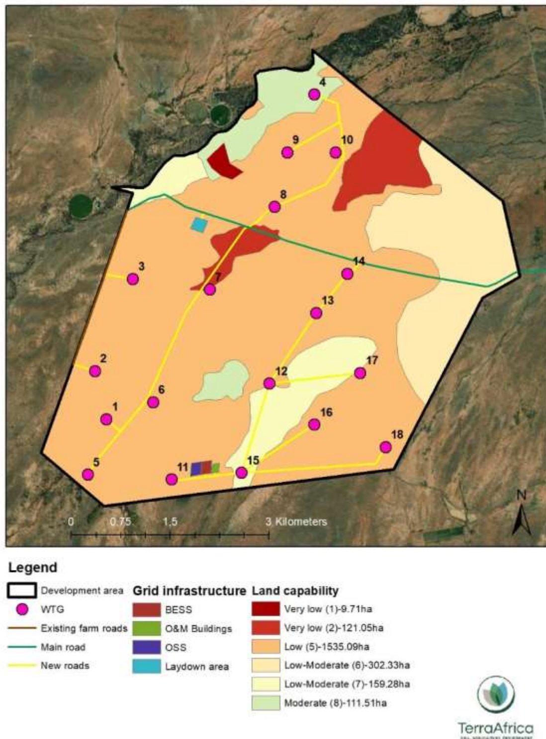
Figure 10: Land capability classification of the Tango Wind Energy Facility development area.
