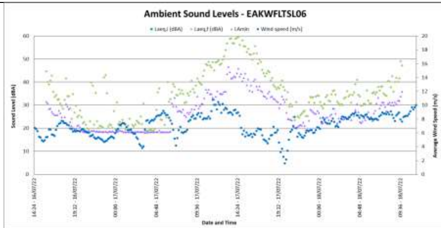
Figure 4-25: Ambient Sound Levels at EAKWFLTSL06
