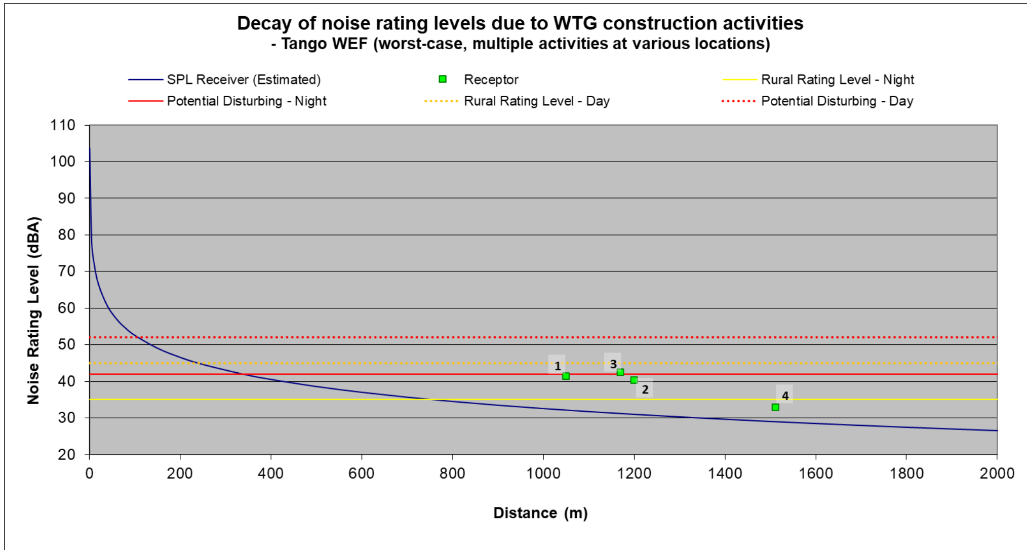
Figure 9-3: Projected conceptual construction noise levels for the proposed FE Tango WEF
