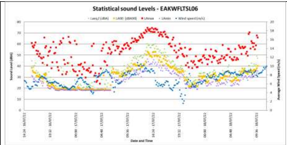
Figure 4-26: Maximum, minimum and Statistical sound levels at EAKWFLTSL06
