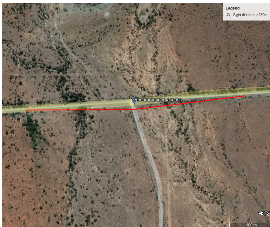
Figure 5-9: Shoulder Sight Distances on MR00599 from Access point
