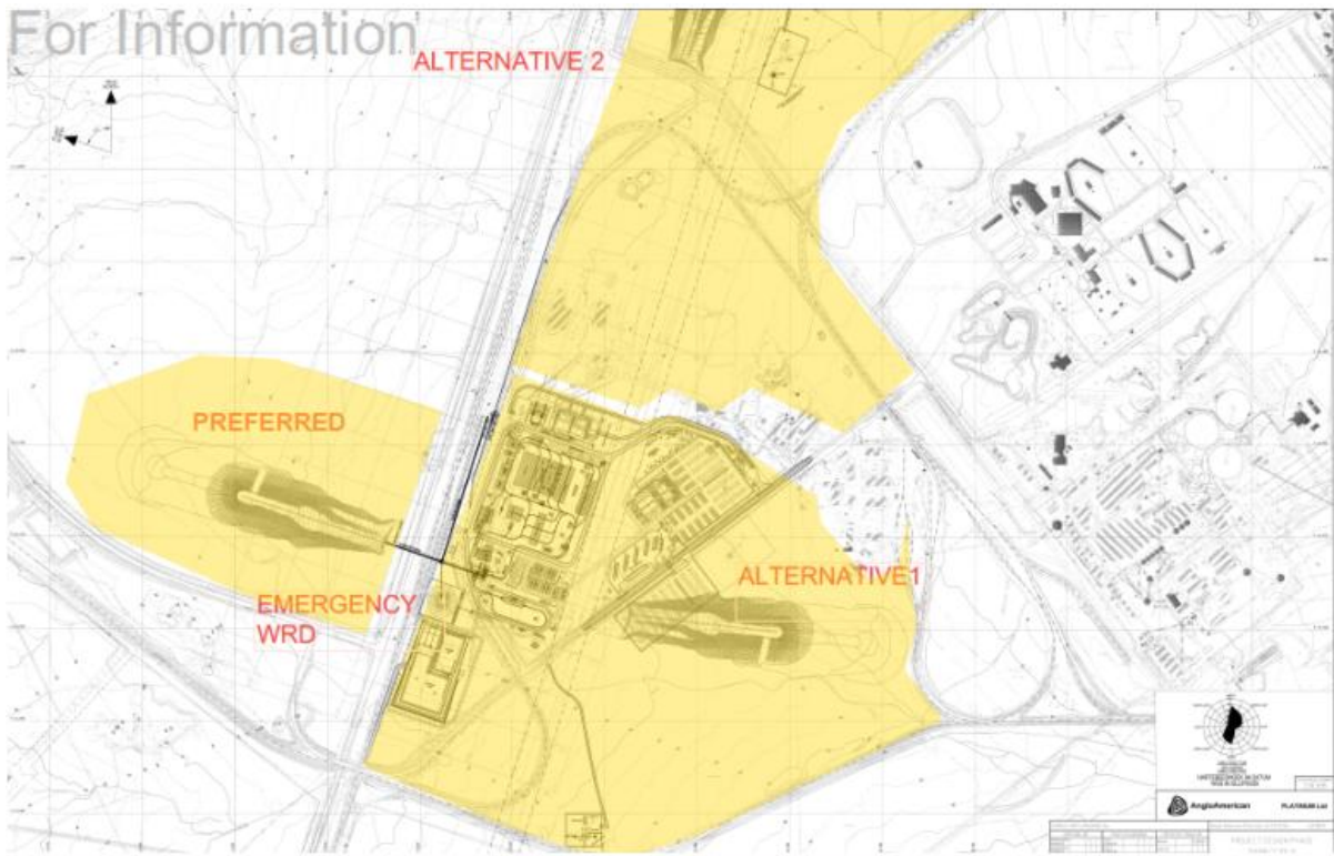
Figure 4 Proposed layout of the Central Shaft and the different options for the Waste Rock Dump.
