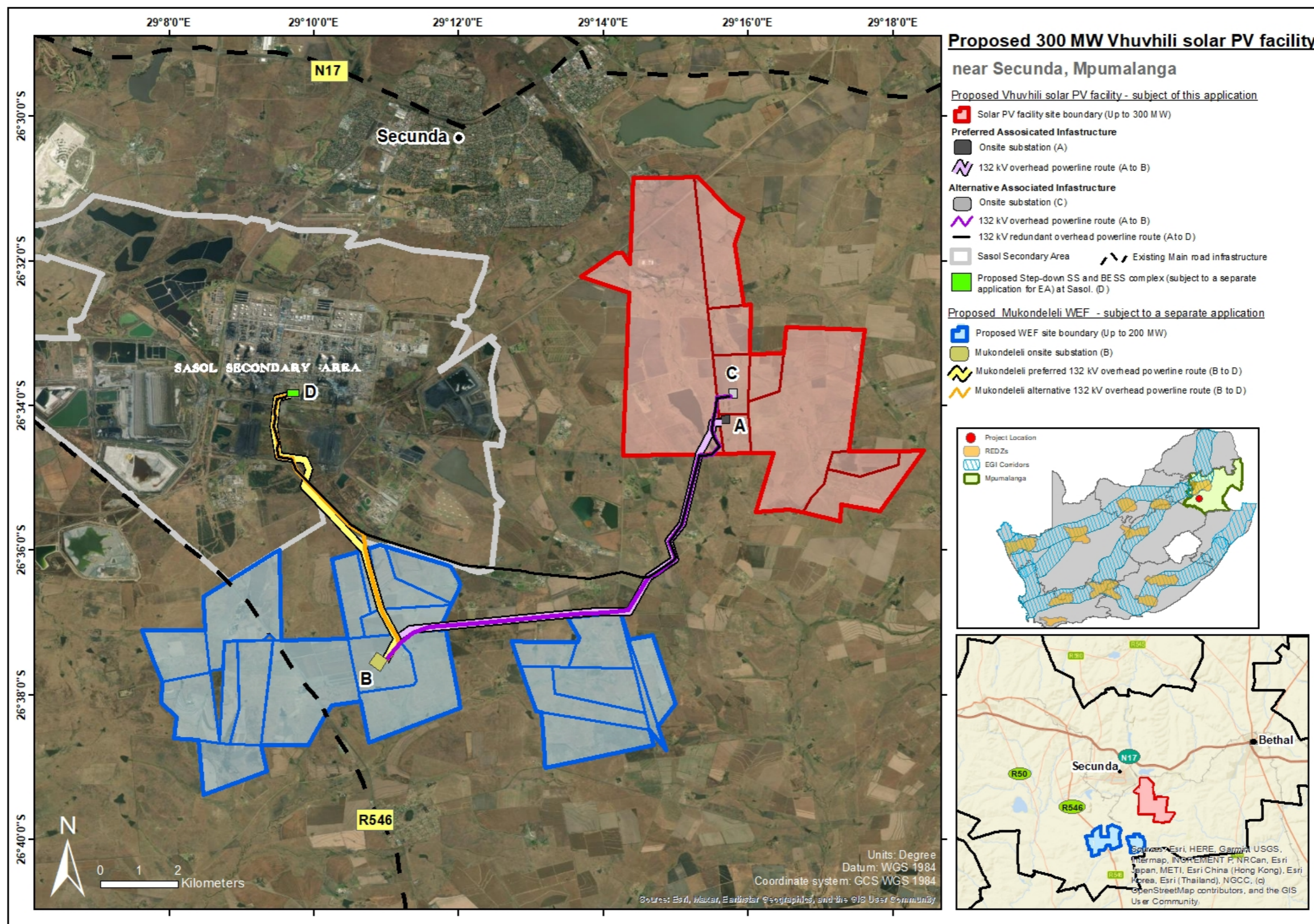
Figure 3: Proposed Power Line and Electrical Grid Infrastructure associated with the proposed Vhuvhili Solar PV Facility (subject to a separate Environmental Assessment application).
