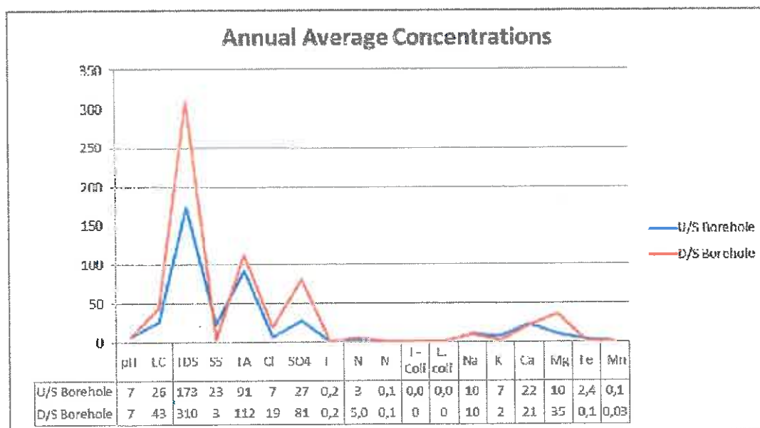
Figure 4-3: Annual Average Concentration for all Groundwater Monitoring Points
