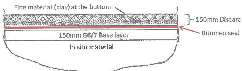
Figure 9: Sealing arrangement for the stockpiles
