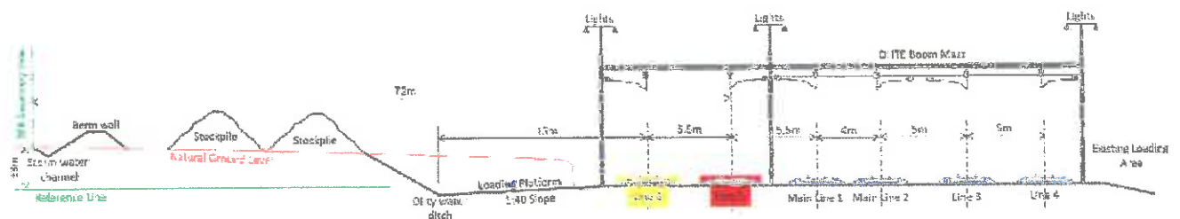
Cross-section of the siding for phase 1
