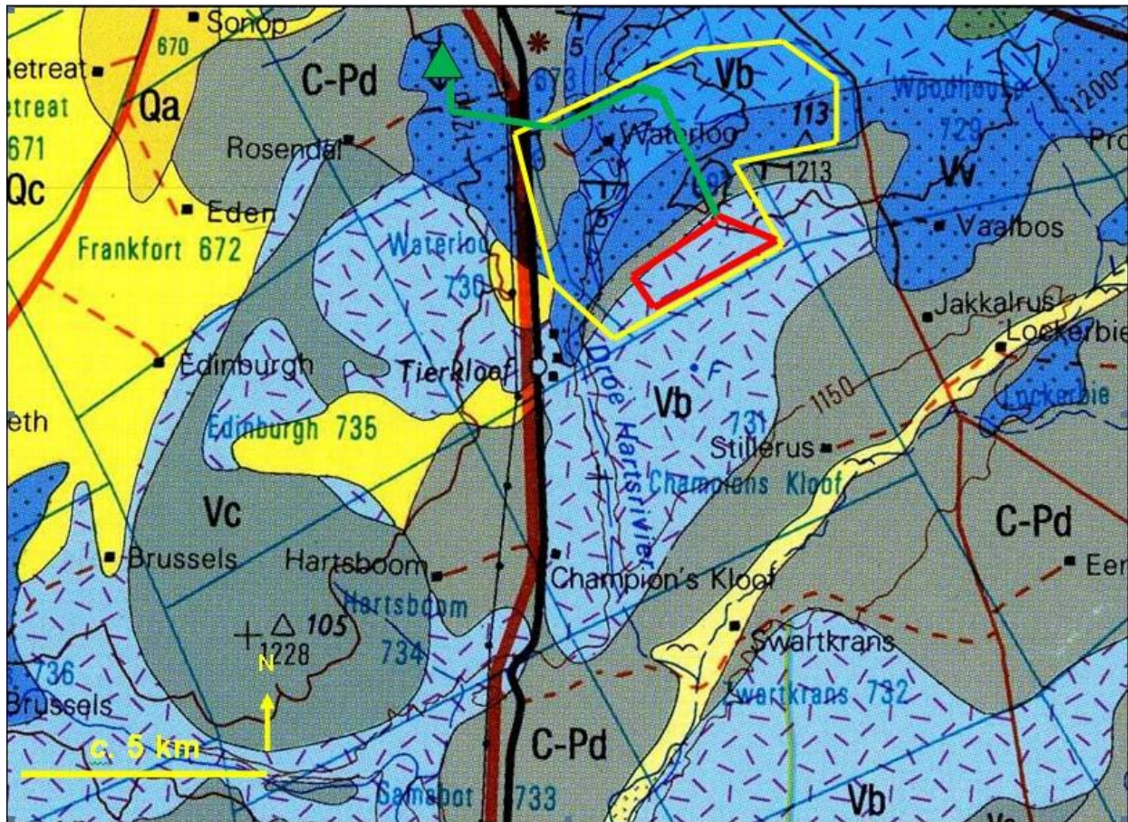
Fig. 3. Extract from the 1: 250 000 geological map 2724 Christiana (Council for Geoscience, Pretoria) showing location of the broader study area on the farm Waterloo 992, located some 10 km southeast of Vryburg (yellow polygon). The red polygon shows the expanded solar development area and the green line indicates the approximate power line route to Mookodi Substation (green triangle).
