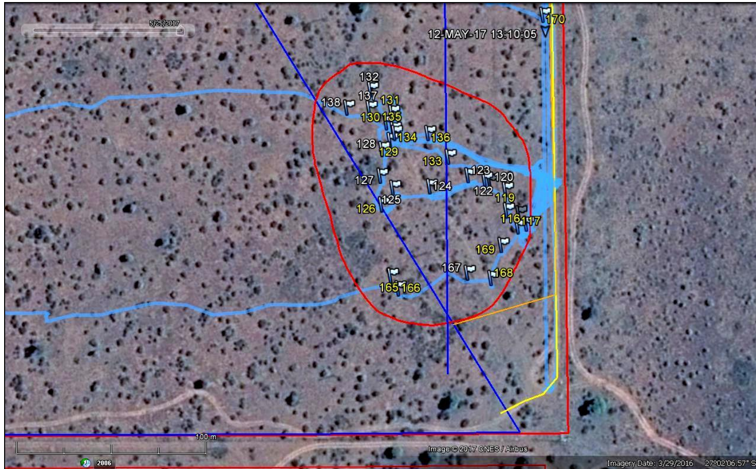
Fig. 39. Satellite image of eastern corner of the study area (N towards top right). The area outlined in red includes a high concentration of large domal stromatolites (yellow waypoints) that lies largely outside and to the east of the main solar facility development area (dark blue polygon shown in previous figure). Access road Alternative 1 (unmitigated) is shown in dark blue and the existing farm track in yellow. The yellow access road is preferred from a fossil heritage point of view. However, a mitigated version of the Alternative 1 route (orange in this and the following figure) is also acceptable since it avoids the palaeontologically-sensitive area outlined in red. During construction the protection - e.g. by fencing or security tape - of stromatolites exposed at surface within the portion of the red area that lies outside the main solar facility development area is recommended. Most of the stromatolite sampling took place within this red-outlined area.
