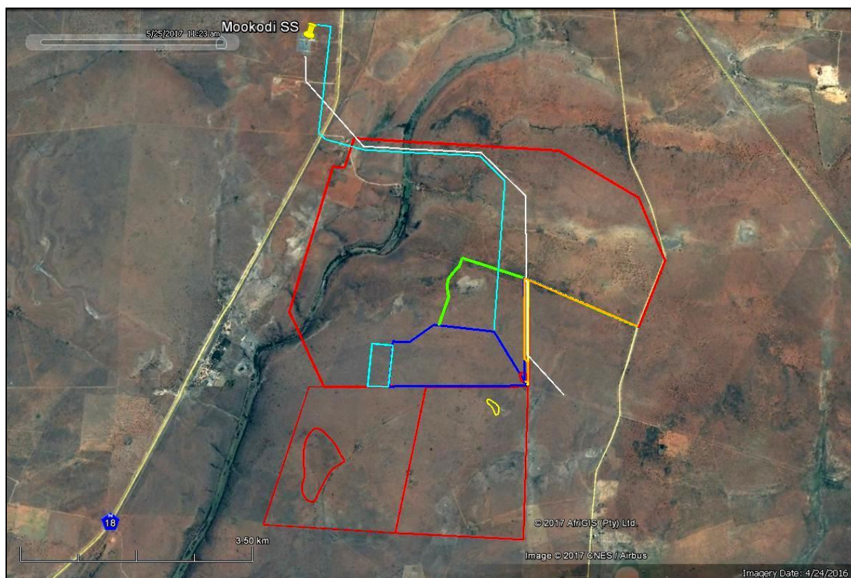
Fig. 2. Google earth© satellite image of the broader study region to the south of Vryburg, Northwest Province. Note N is towards the top right in this view.
