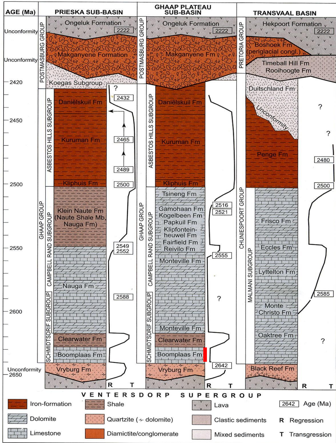
Fig. 4. Stratigraphy of the Transvaal Supergroup of the Ghaap Plateau Basin (central column) showing the position of the carbonate-dominated Boemplaas Formation that underlies the Waterloo Farm 992 solar energy facility main project area (red line) (From Eriksson et al. 2006). The proposed access road to the solar facility will in addition traverse the outcrop area of quartzites and lavas of the underlying Vryburg Formation (also included within the Schmidtsdrif Subgroup by some recent authors).
