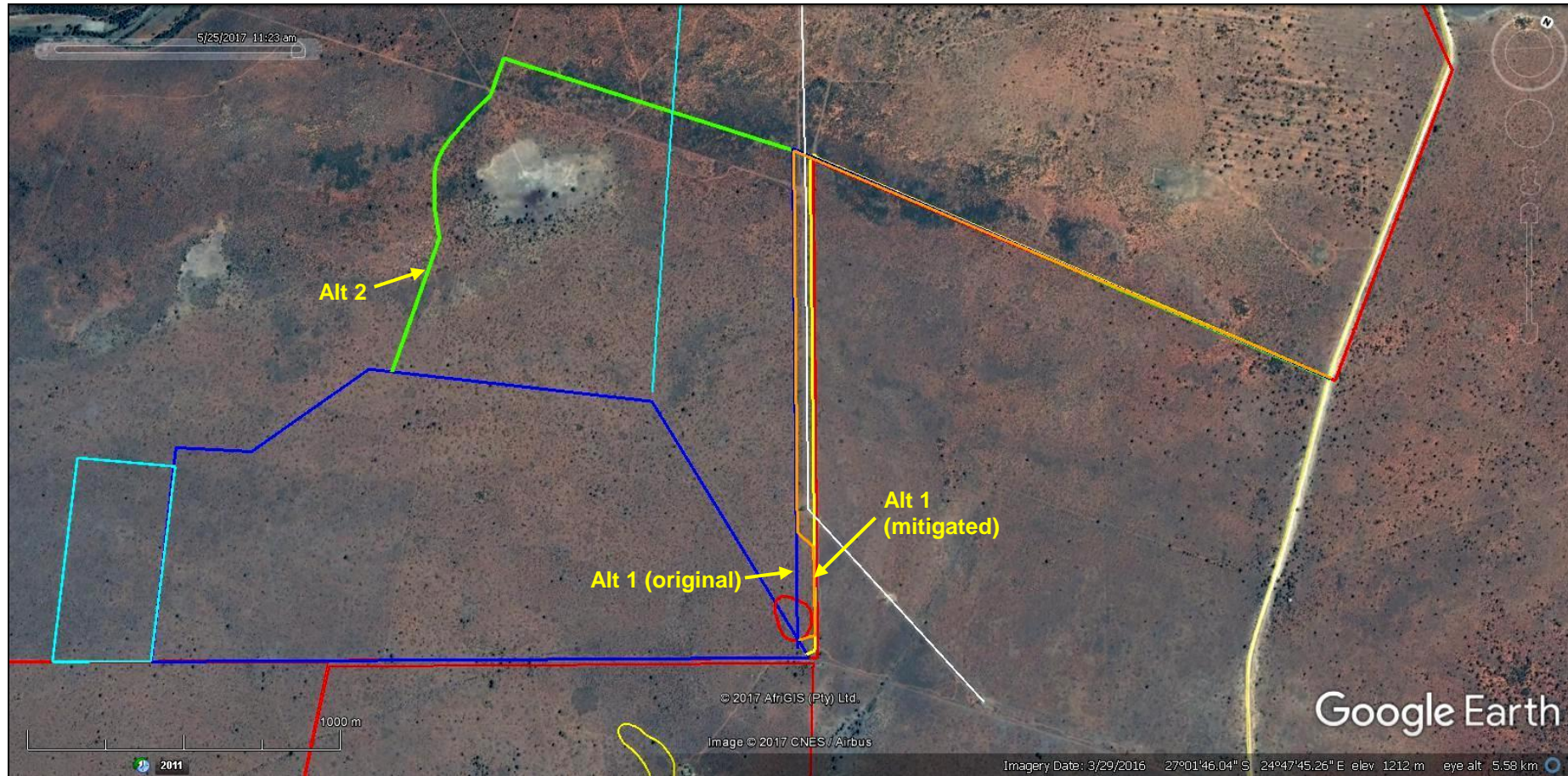
Fig. 40. Google earth© satellite image of the solar facility study area on Waterloo Farm 992 showing the two access route options under consideration. Alternative 1 runs parallel to and slightly west of the farm boundary (blue). Alternative 2 (green) skirts a pan to the north of the main solar project area. A mitigated version of Alternative 1 (orange) has been proposed in order to avoid the sensitive stromatolite-rich area (red circle). This last is the preferred option from a palaeontological heritage viewpoint. An existing farm track (yellow) runs along the eastern boundary of the property.
