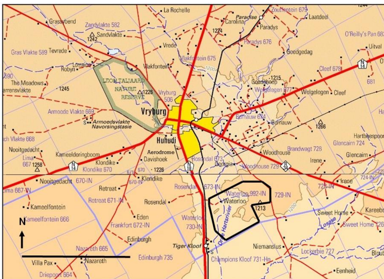
Fig. 1. Extracts from adjoining 1: 250 000 topographical maps 2624 Vryburg and 2724 Christiana (Courtesy of the Chief Directorate of Surveys & Mapping, Mowbray) showing location of the farm Waterloo 992 study area some 10 km southeast of Vryburg, North-West Province (black polygon). Scale bar is c. 10 km. Important Precambrian stromatolite occurrences are also known on the farm Champions Kloof 731 immediately to the south.
