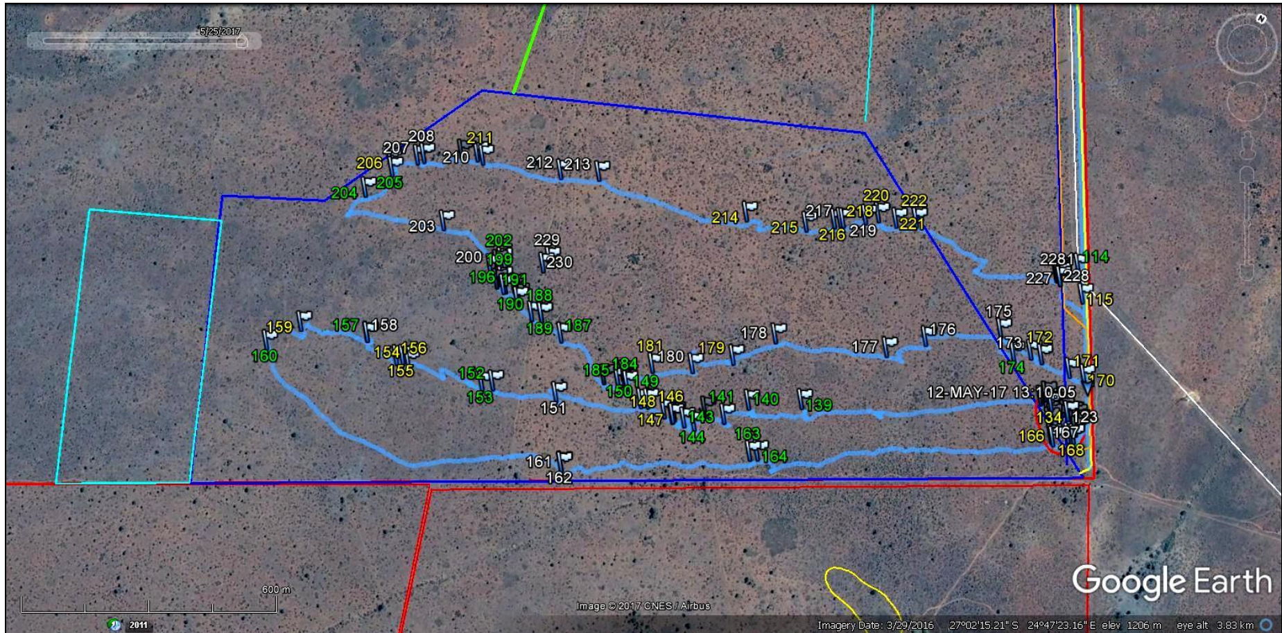
Fig. 38. Google earth© satellite image of the main solar facility study area on Waterloo 992 (dark blue plus pale blue) showing gps tracks and numbered waypoints recorded during fieldwork in May 2017 (Note N is towards the top right of the image). Most of the waypoints refer to stromatolite occurrences within the Boomplaas Formation which clearly occur widely across the area. Their apparent distribution is probably largely governed by low levels of bedrock exposure rather than being an original feature (e.g. patch reefs). Yellow waypoints = large domal stromatolites. Green waypoints = medium-sized stromatolites (domes / short columns). White waypoints = other features (e.g. stromatolite buttons, geological phenomena) (Please see Appendix 1 for details).
