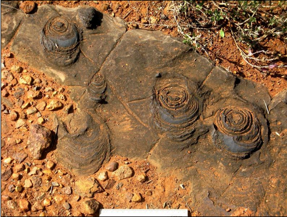
Fig. 29. Well-spaced, concentrically-laminated stromatolites with an ellipsoidal plan showing asymmetric growth towards the observer (Scale is 15 cm long). Note smooth lamination surfaces here (Loc. 196).
