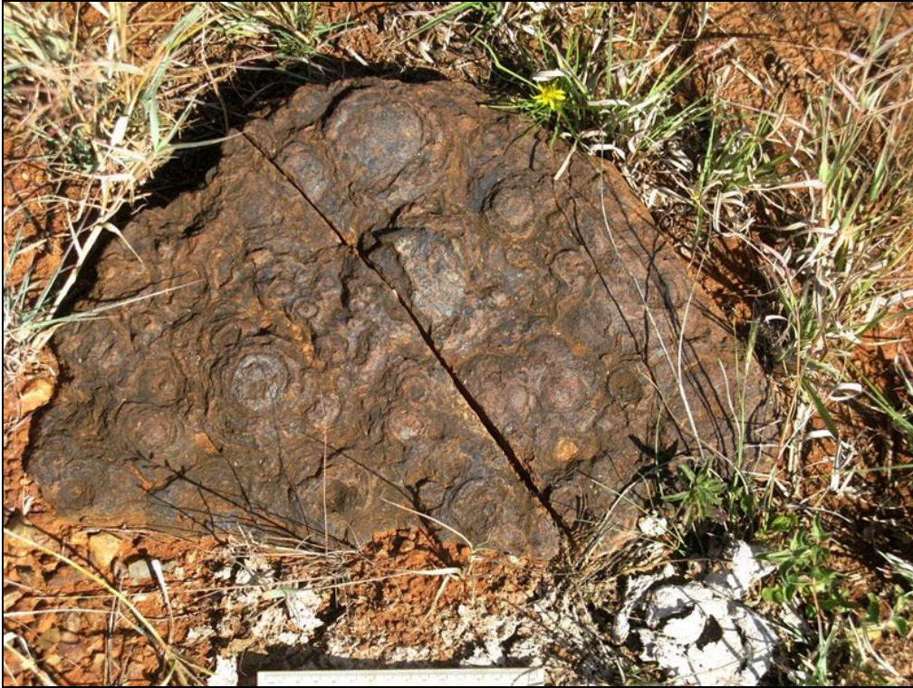
Fig. 31. Bedding plane of ferruginous carbonate covered with small-scale stromatolitic microdomes of various diameters (Scale in cm) (Loc. 210).
