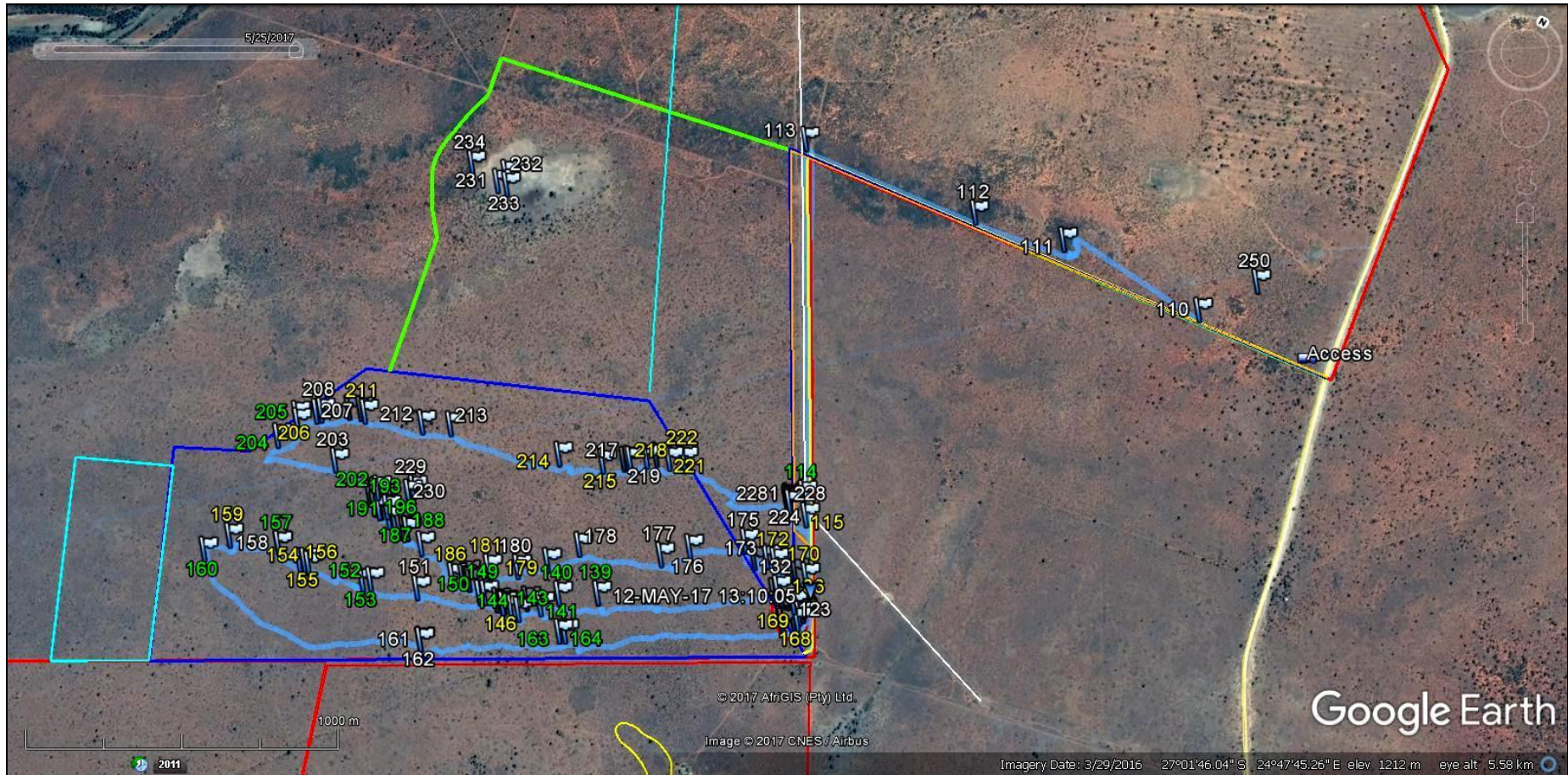
Fig. 37. Google earth© satellite image showing the outline of adjoining Farms Waterloo 992 and Champions Kloof 731 near Vryburg (red), the expanded solar facility study area (dark blue plus light blue polygons). Close-up images showing tracks and waypoints in more detail are provided in Figs. 38 & 39 while access road options are shown in Fig. 40. N.B. North is towards the top right of the image.
