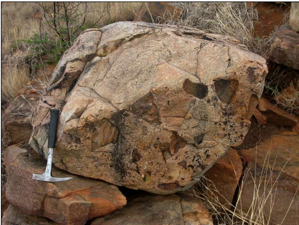
Fig. 6. Intraclast breccia with angular moulds of reworked mudrock on a quartzite sole, lower Vryburg Formation (Hammer = 29 cm).
