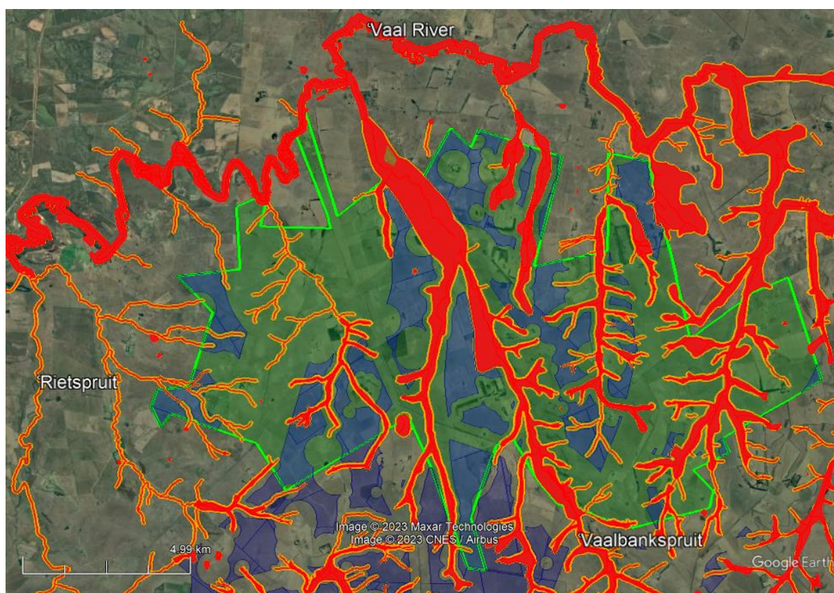
Figure 15. Google Earth image showing the aquatic sensitivity mapping together with the proposed layout (buildable areas) for the project for the site.
