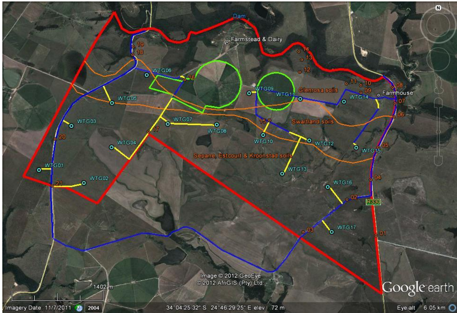
Figure 14.2b: Site Plan of Banna Ba Pifhu Wind Farm for alternative 2, the preferred alternative (30.6 MW, 17 turbines). Turbine positions and numbers in light blue, existing roads in blue, new roads in yellow, irrigation lands outlined in green, soil lines and sample numbers in light brown. Details of all soil sample points are provided in Appendix 14.1
