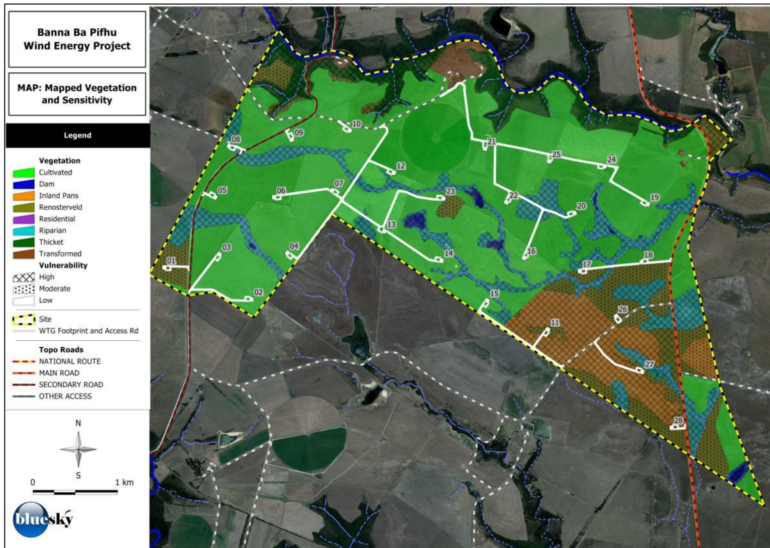
Figure 5-41: Mapped Vegetation communities with Alternative 1 50 MW layout overlain for maximum number of sites (28 turbines).
