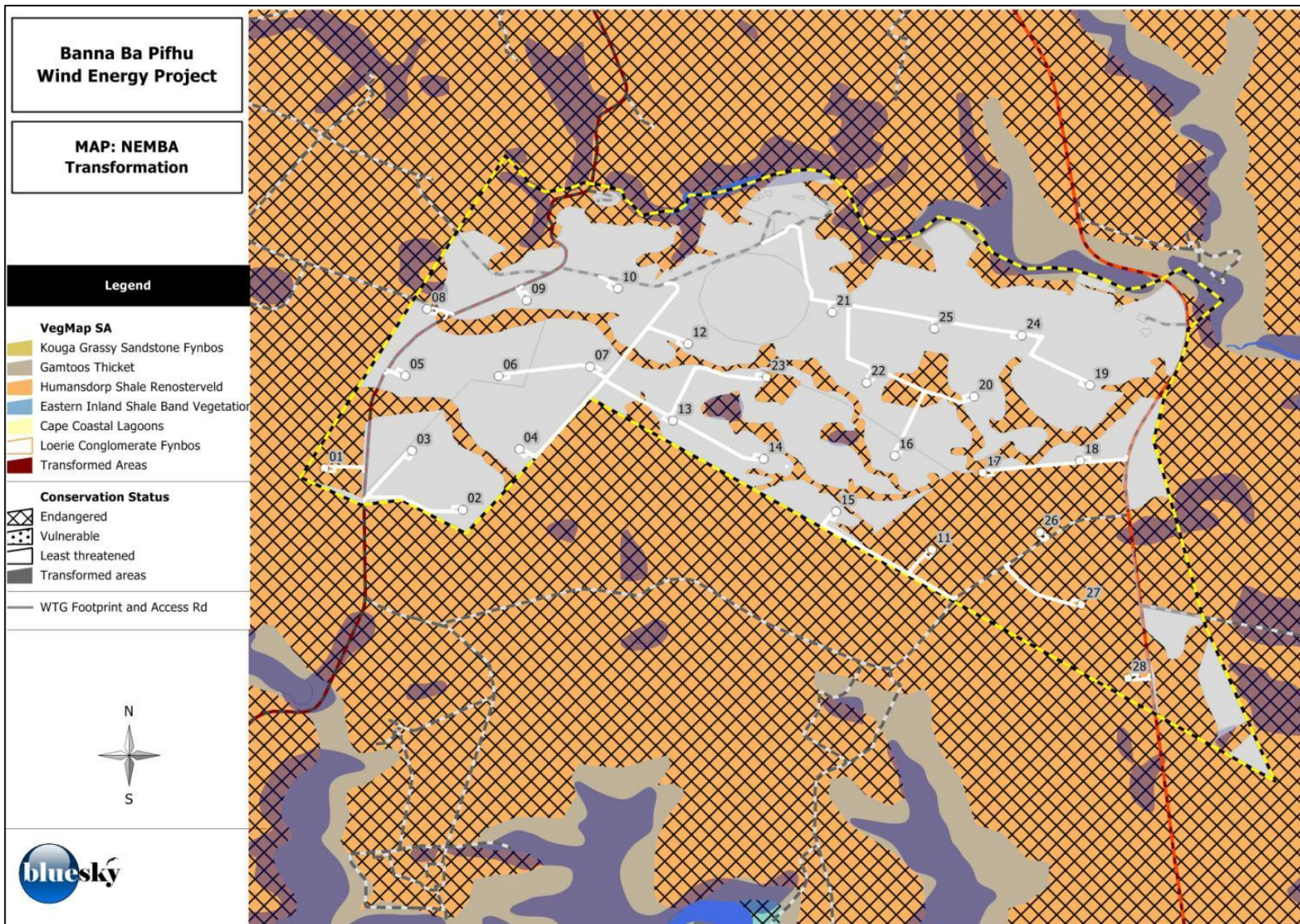
Figure 5-7: Alternative 1 (50 MW) site layout plan indicating turbine sites affected by NEMBA. Transformed areas indicated in grey.
