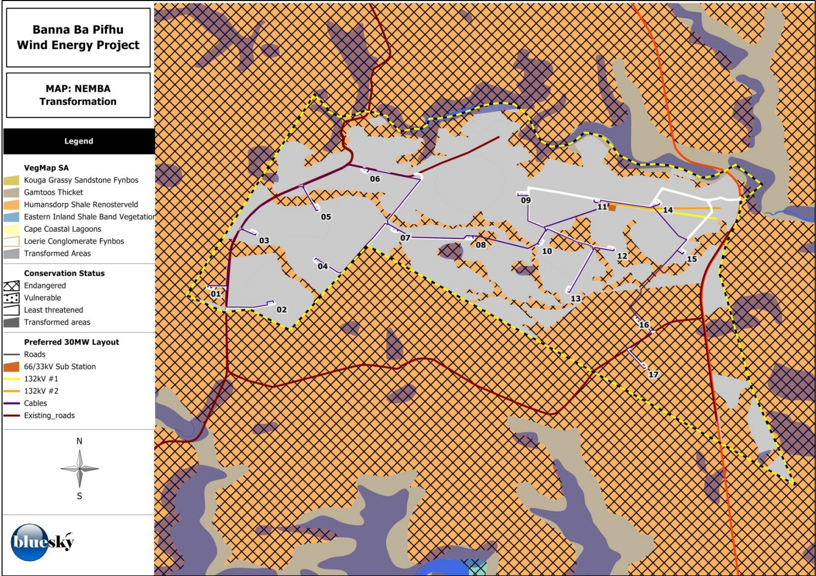
Figure 5-6: Preferred Alternative (30.6 MW) site layout plan indicating turbine sites affected by NEMBA. Transformed areas indicated in grey.
