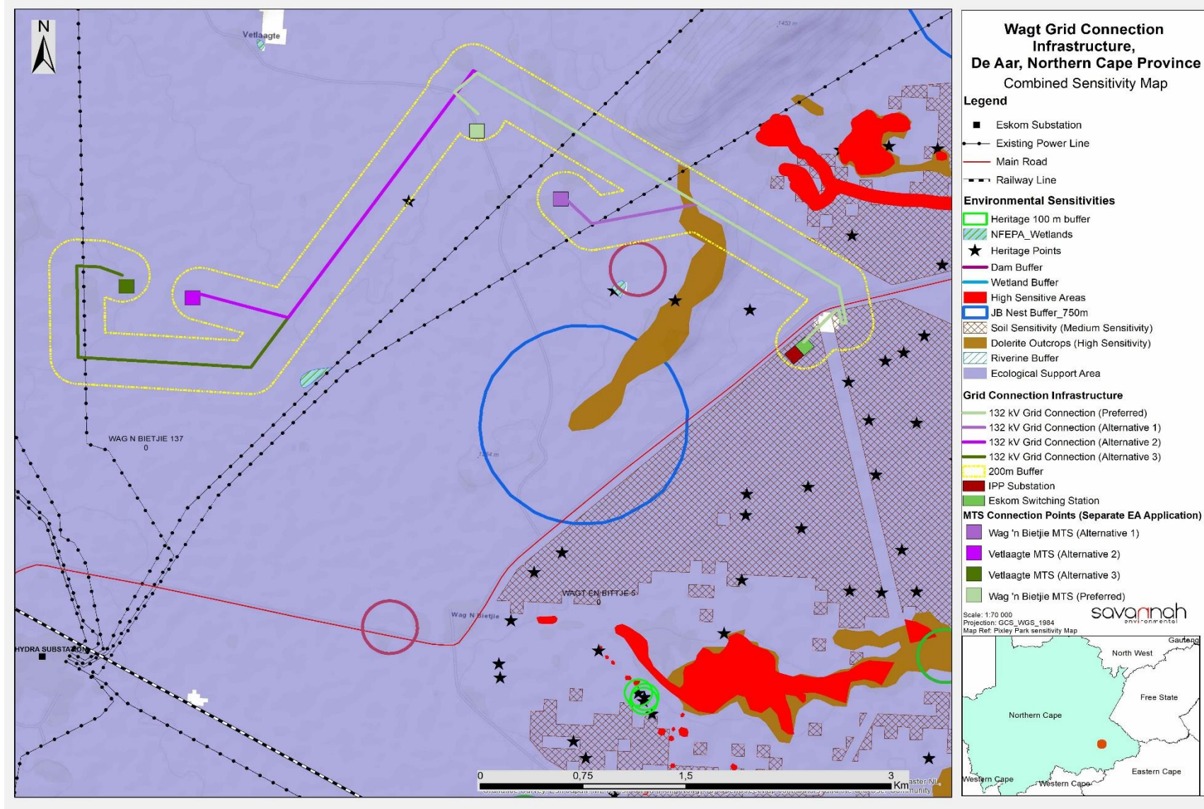
Figure 1: Environmental sensitivity map showing the grid connection corridor and collector substation location
