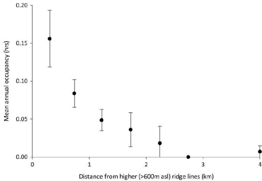
Figure 18. Verreaux's Eagle flight density and distance from higher (>600m) ridge lines, Choje East June 2019 - August 2020 (mean ± 95% confidence limits).
