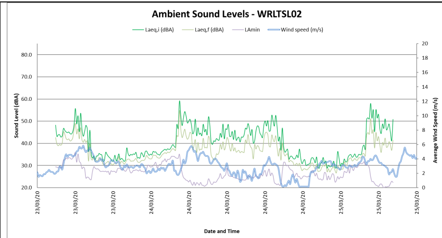
Figure 4-10: Ambient sound levels at WRLTSL02
