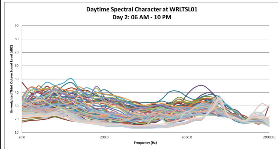
Figure 4-7: Spectral frequencies - WRLTSL01, Day 2
