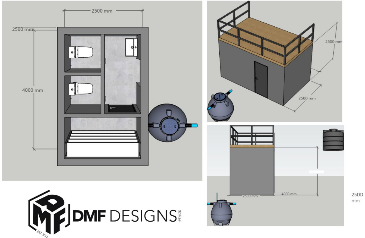
Figure 3: Ablution design proposed for Gladysvale Cave.
